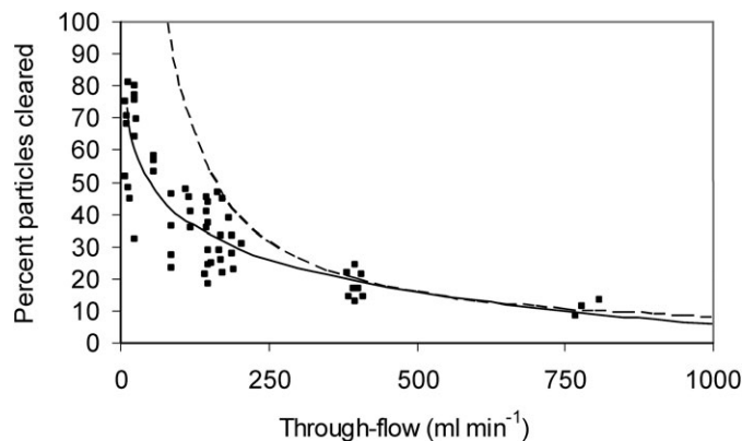
Fig. 4. Flow-through chamber (FTC) method. Percent particles cleared, 100 \times P = 100 \times (C_i - C_o)/C_i , versus chamber through-flow, Fl . Full line: logarithmic fit (Filgueira et al., 2006; their Fig. 5, re-plotted); dashed line: hyperbolic function, CR_m/Fl , for ideal chamber and CR_m = 78.87 \text{ ml min}^{-1} .
