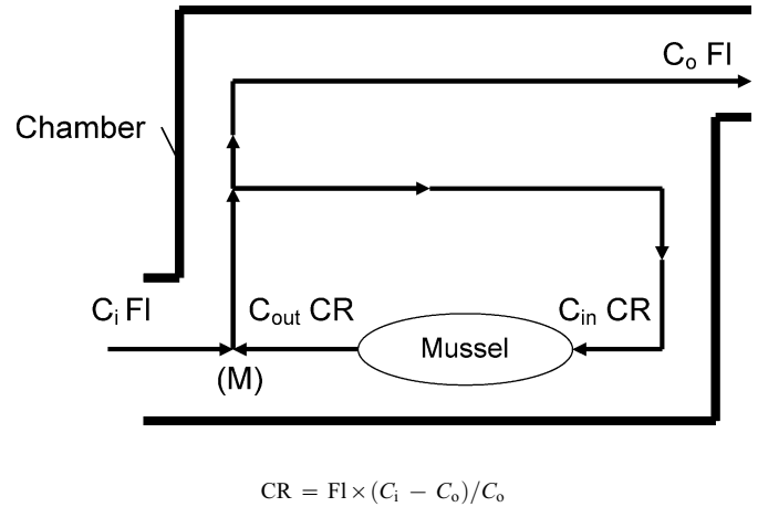
Fig. 2. Diagram of the steady-state (SS) method. (M) denotes point of perfect mixing. C_i and C_o denote concentration of chamber inflow and outflow, respectively, C_{in} ( = C_o ) and C_{out} ( = 0 for 100% retention) the concentration of inhalant and exhalant flows, respectively, FI the chamber through-flow, and CR the clearance rate given by Eq.(2).
