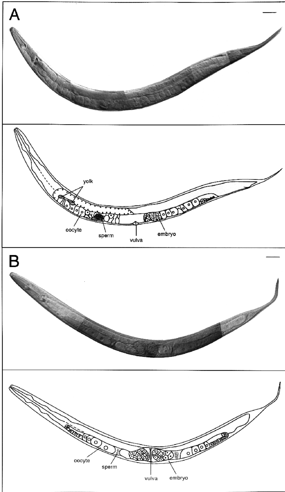
Fig. 3. XO tra-2(eg) mutants are transformed from male to hermaphrodite. (A) Top, Nomarski DIC photomicrograph (400×) of adult XO tra-2(e2531eg) hermaphrodite, lateral view. Bottom, schematic representation of photomicrograph. (B) Top, For comparison, Nomarski DIC photomicrograph (400×) of adult wild-type XX hermaphrodite, lateral view. Bottom, schematic representation of photomicrograph. Scale bar, 20 μm.
