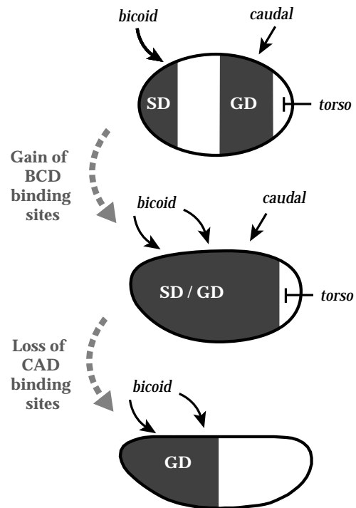
Fig. 6. Model for the evolution of the hunchback expression pattern. Top: hunchback expression in Tribolium , which represents the ancestral state. Regulation of the serosa domain by bicoid and regulation of the gap domain by caudal and torso is indicated. Center: hypothetical intermediate state. A large expression domain is formed by fusion of the two initial domains due to insertion of additional bicoid sites. Bottom: in Drosophila , the large gap domain is in the anterior half. This situation could be due to the loss of caudal activation, thereby shifting the posterior border of the domain towards the anterior.
