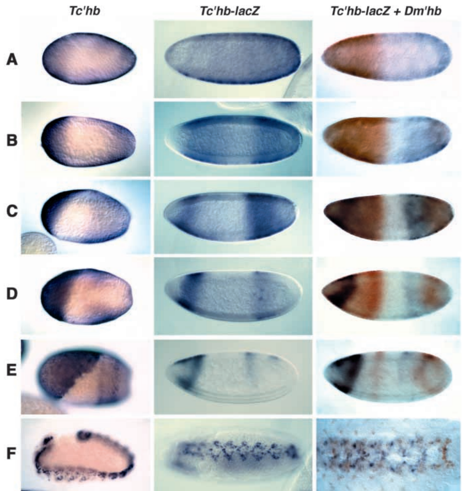
Fig. 2. RNA expression of the Tc'hb-lacZ reporter gene in Drosophila (central column). For comparison, Tc'hb expression in Tribolium is also shown (left column), and in the right column Drosophila embryos are pictured which are doubly stained for the reporter gene and endogenous Dm'hb . The reporter gene includes 5 kb of Tc'hb upstream DNA. A-F represent embryos of similar developmental stages across the columns. Early in the syncytial blastoderm, the reporter gene initiates near homogeneous expression (A) which resolves into two domains of which the posterior includes the posterior pole (B). During cellularization, these domains contract somewhat, and the posterior domain retracts from the pole similarly to Tc'hb (C,D). At the end of the cellular blastoderm, the posterior domain dissolves into two stripes and finally disappears (E). In the fully extended germ band, expression in the ventral nerve cord becomes apparent in Drosophila and Tribolium (F). The double in situ staining in the right column demonstrates that the reporter gene initiates expression coincidentally to the endogenous Dm'hb gap domain, and it shows that the reporter gene is expressed in a subset of CNS cells which also express the endogenous Dm'hb gene. The Drosophila embryos in F are ventral views.
