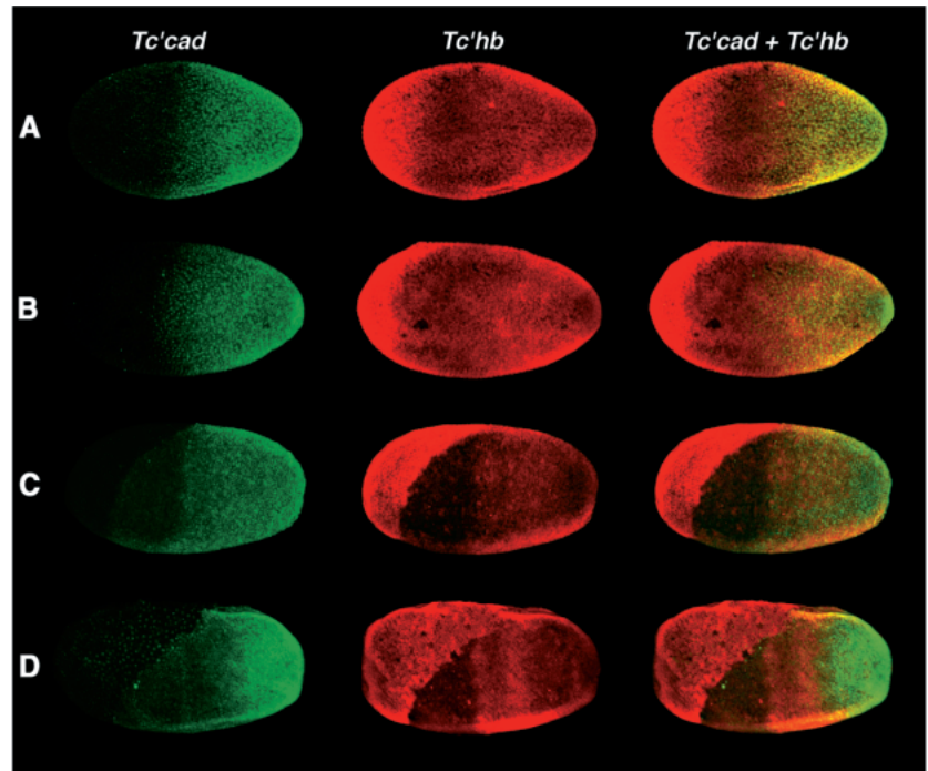
Fig. 5. Overlap of Tc'cad and Tc'hb mRNA expression domains in Tribolium embryos of successive developmental stages. (A,B) blastoderm stages; (C,D) formation of the germ rudiment. The anterior domain of Tc'hb demarcates the serosa primordium which expands during germ rudiment formation as embryonic cells move towards ventral and posterior regions. The posterior domain (which has a lower expression) arises within the Tc'cad domain. During germ rudiment formation, this domain weakens and resolves into two stripes, while the Tc'cad domain retracts towards the region of the prospective growth zone at the posterior pole (D).
