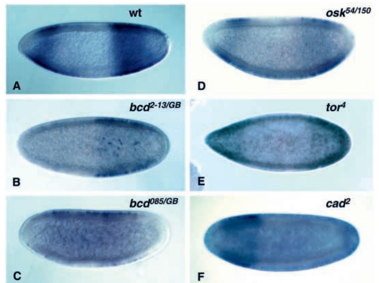
Fig. 3. Regulation of Tc'hb-lacZ by Drosophila segmentation genes. (A) Wild-type embryo. (B) In embryos of reduced bicoid activity ( bcd 2-13 /bcd GB ), the anterior domain is lost and the posterior domain expands anteriorly. (C) In a combination of strong bicoid alleles ( bcd 085 /bcd GB ), the posterior domain expands almost to the anterior pole. (D) In oskar 54/oskar 150 embryos, the size and position of the two domains is unaffected. (E) In torso 4 , both the anterior and the posterior domains fail to retract from the poles. (F) The posterior domain of Tc'hb-lacZ is missing in embryos maternally mutant for Dm'cad . In B-F, the amount of transcript is reduced relative to A because only one copy of the transgene was present in mutant backgrounds.
