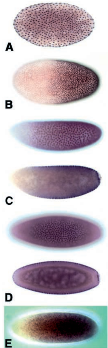
Fig. 1. Expression of Tc'CAD protein in Tribolium and Drosophila . (A,B) Distribution of Tc'CAD in early and late blastoderm embryos in Tribolium . (C) Expression of Tc'CAD protein in transgenic Drosophila embryos (two focal planes are shown). Maternally expressed Tc'cad mRNA is homogeneously distributed (not shown); anterior repression of Tc'cad translation therefore indicates posttranscriptional regulation. (D) Two focal planes of a embryo carrying the same construct, but in a bcd E1 /bcd GB mutant background. In this situation, all blastoderm nuclei, including the anterior pole, express Tc'CAD protein. (E) A protein gradient is also formed in unfertilized Drosophila eggs (genotype as in C), indicating that this regulation is not mediated by zygotic target genes of bcd . As in the other figures, embryos are oriented dorsal up and anterior to left.
