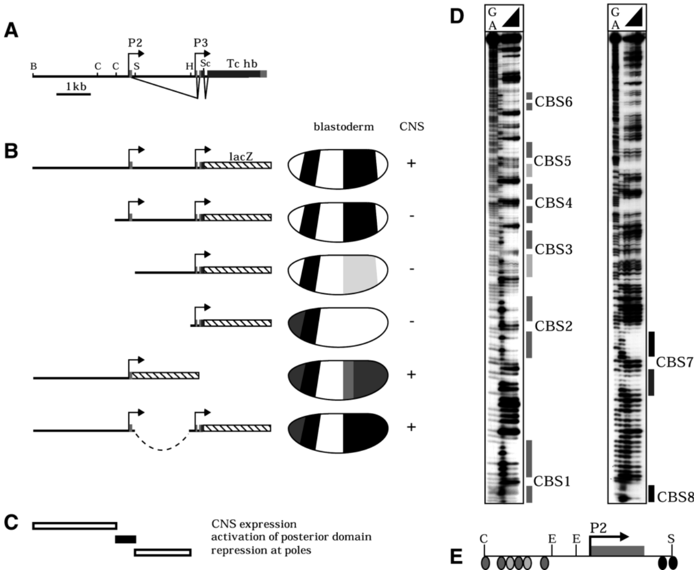
Fig. 4. Identification of a Tc'hb upstream fragment required for activation of the gap domain, and identification of CAD binding sites within this fragment. (A) Map of the Tc'hb locus. The region depicted includes two of the three promoters (P2, P3). The coding region (black) is interrupted by a short intron. Transcripts starting at P2 and P3 are spliced to the same coding sequences via introns in the untranslated regions (gray; Wolff et al., 1995). (B) Upstream fragments contained in different reporter gene constructs. lacZ mRNA expression from these construct is indicated to the right, i.e. expression in the blastoderm stage (embryo sketches) and presence/absence of CNS expression (+/-). (C) These constructs identify a region of 560 bp which is required for the caudal -dependent posterior domain of Tc'hb-lacZ (black box). In addition, a region required for repression near the poles is indicated, as well as a region required for expression in the CNS. The anterior domain is present in all constructs tested, indicating that sites mediating activation of this domain by bicoid may be dispersed throughout the region. Alternatively, the anterior domain in these lines could be due to sites in the transformation vector. Such artifactual anterior expression has occasionally been observed with pCasper vectors (Klingler et al., 1996). However, the anterior domain in our constructs arises much earlier during embryonic development than is the case with this artifactual expression. In addition, we have tested the largest construct in a different transformation vector, pHZ50 (Hiromi and Gehring, 1987), for which no anterior artifact has been described. Expression from this vector was identical to that in embryos carrying the corresponding Casper vector (not shown). (D) Footprinting reactions with bacterially expressed Dm'CAD (Rivera-Pomar et al., 1995). The ClaI-SalI fragment highlighted in C was further cut with EcoRI and the resulting fragments labeled at the ClaI (left panel) and SalI ends (right panel). In each panel, lane 1 is the Maxam-Gilbert reaction, lane 2 is CAD-free control, and lanes 3-5 contain 1, 5 and 10 \mu g of total protein per reaction, respectively. Protected sites are indicated at the side of each panel, each binding site consisting of two half sites (Dearolf et al., 1989a). Strength of protection is indicated by different gray shades. (E) Detail of the same Tc'hb upstream fragment. Ovals indicate the location of protected binding sites as identified in D. Six binding sites are located upstream of the P2 promoter, but the two strongest sites are situated downstream, in the intron (CBS8, CBS9). The sequences of these CAD binding sites (CBS1 to CBS8) are: TCGAAAN 7 CATAAA, ATCTAAN 5 TTTAAC, TTTATTN 3 TTTATT, TTTGGAN 3 TTTATG, ACTAAAN 4 TTTACG, TTTCAGN 4 TTTATT, TTTATTN 5 TTTGCA and AGTAAAN 4 CATAAA. Restriction sites in A and E are B, Bam HI; C, Cla I; E, Eco RI; H, Hind III; S, Sal I; Sc, Sac II.
