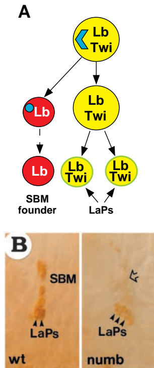
Fig. 6. Divisions of lb -positive progenitor. (A) The lb -positive progenitor divides two times. First, a morphologically asymmetric division leads to the transmission of Nb protein (blue chevron) to the SBM founder. The second division of a progenitor devoid of Numb gives rise to two twi and lb -positive LaPs. (B) The lb staining of wild-type (left, subpanel) and nb - embryo (right, subpanel) shows the formation of a supernumerary LaP and absence of SBM (open arrow) in nb - background. In these embryos, all progeny of lb -positive progenitors are devoid of Nb and become LaPs.
