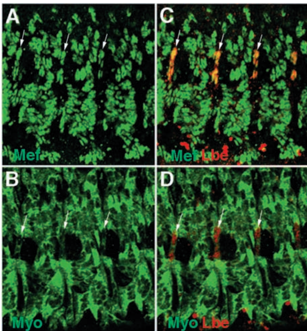
Fig. 1. lb expression is associated with the SBM. (A-D) Confocal scans of the ventrolateral part of stage 16 embryos double stained for Lbe and two muscle markers: Mef2 and Myosin. (A,C) Myoblast nuclei labelled using anti-Mef2 antibody (green) and (C) anti-Lbe antibody (red). SBM nuclei (arrows) that co-express Mef2 and Lbe appear yellow. (B,D) The muscle fiber architecture stained with anti-Myosin (green) and (D) myoblasts expressing lbe (red). The lbe -positive myoblast nuclei are associated with only one muscle fiber per segment, the SBM (arrows).
