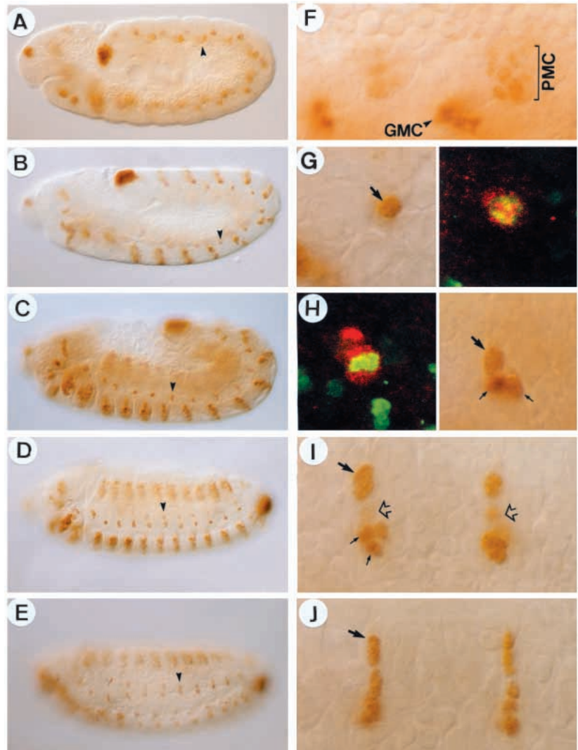
Fig. 3. SBM fiber formation. (A-J) Immunostainings of embryos with anti-Lbe antibody. (F-J) Higher magnification of lb -positive myoblasts indicated on A-E by arrowheads. (A,F) SBM promuscular clusters. (B,G) SBM progenitor (arrow in left G subpanel). (Right G subpanel) Confocal view of the early phase of the first asymmetric division of the progenitor, double stained for Lbe (red) and for Phospho-Histone H3 (green), which labels condensed chromatin in dividing cells. Areas with the overlapping red and green staining appear yellow. (C,H) Divisions of progenitor. (Left H subpanel) Confocal view stained as for the right G subpanel showing the nucleus of SBM progenitor at the beginning of its second division (with the green/yellow chromatin) and its first progeny, the SBM founder (red). (Right H subpanel) The progeny of progenitor after its second division: the SBM founder cell (arrow) and two LaPs (small arrows). (D,I) Fusion of the SBM founder cell with its neighbouring myoblasts (open arrows). Note that after the second asymmetric division the SBM founder migrate dorsally (compare H and I) while the LaPs remain at their original position (small arrows). (E,J) Newly formed syncytial fibers. Developmental stages of the embryos: (A,F) stage 10, (B,G) early stage 11, (C,H) early stage 12, (D,I) stage 13, (E,J) stage 15. In all panels anterior is to the left and dorsal is up. Abbreviations: GMC, ganglion mother cell; PMC, promuscular cluster.
