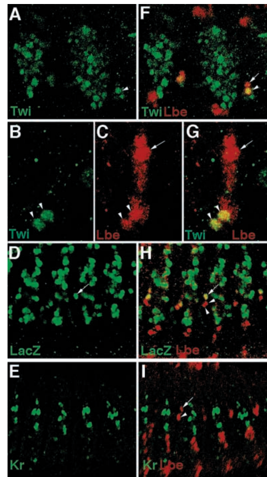
Fig. 2. lb -positive progenitor gives rise to the SBM founder cell and two LaPs. Confocal scans of embryos double stained for lbe (red) and three other markers ( twi , lacZ and Kr ) (green) expressed during early myogenesis. Myoblasts that co-express lb and other markers appear yellow. (A,F) At late stage 11, lbe is co-expressed with twi in only one muscle progenitor (arrowhead), which divides giving rise to the SBM founder cell (arrow). (B,C,G) At stage 14, after second division of the progenitor, two LaPs (arrowheads) co-express twi and lb . The lb -positive founder (arrows) migrates dorsally and fuses with neighbouring myoblasts. lb expression in two distinct myoblast lineages appears confirmed (D,H) by a double staining of an enhancer trap line rP298 (Nose et al., 1998) in which lacZ is co-expressed with lb in most laterally located SBM founder (arrows) but is not in two LaPs (arrowheads). (E,I) Kr is expressed in muscle precursors located close to the lb -positive SBM founder (arrow) and LaPs (arrowhead).
