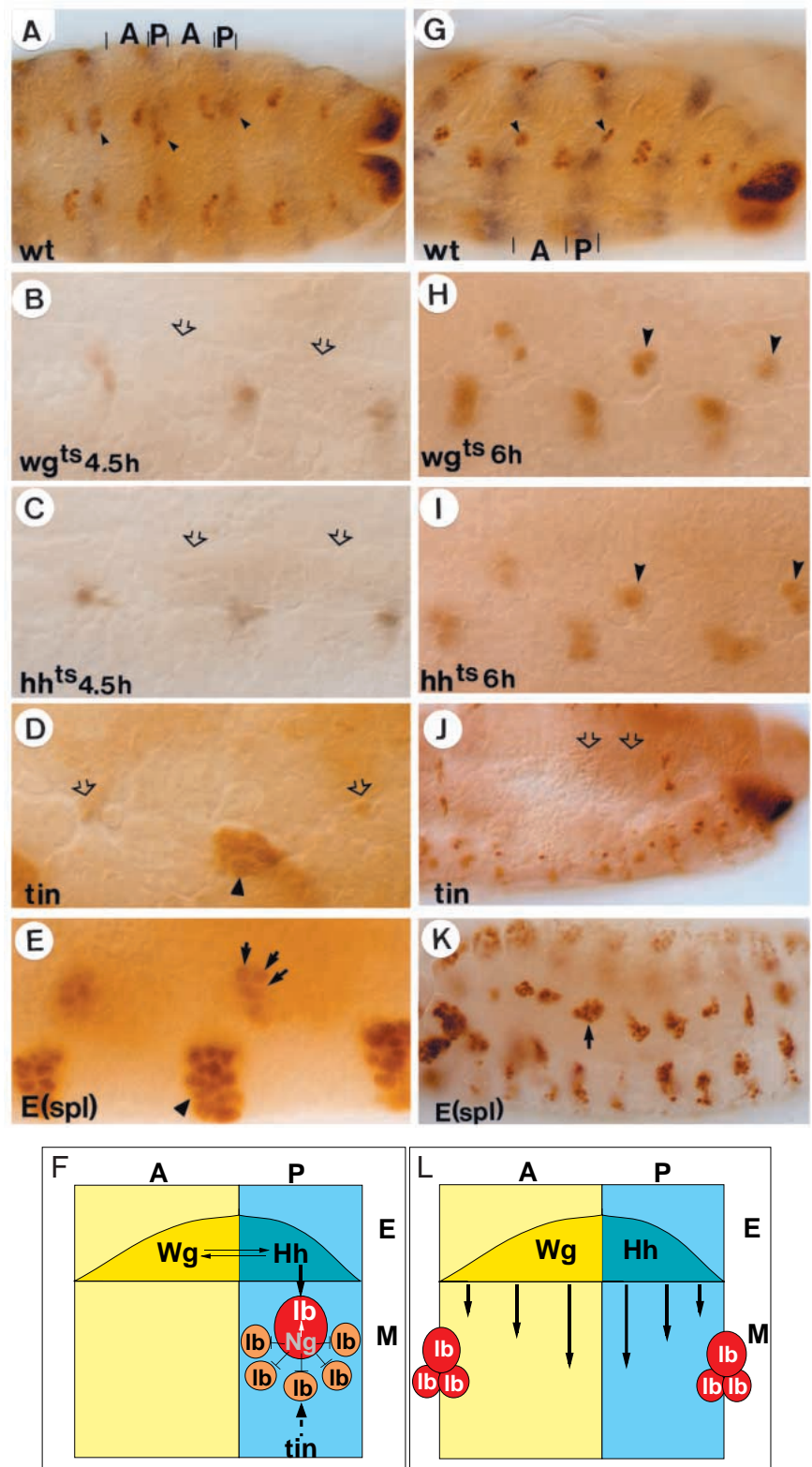
Fig. 4. Mesodermal and epidermal factors contributing to the specification of SBM progenitor. (A,G) Embryos double stained with anti-Lbl antibody (orange/brown) and with anti-Engrailed antibody (blue), which labels the epidermal posterior (P) compartment. Arrowheads point to lb -positive promuscular clusters. (B) lb -positive cells are absent (open arrows) in wg ts and (C) hh ts embryos shifted to the non-permissive temperature at 4.5 h AEL. (H,I) The temperature shift at 6 hours AEL has no effect on lb expression in SBM precursors (arrowheads). (D,J) In tin - embryos, the SBM promuscular clusters and the majority of SBM fibers are absent (open arrows). The arrowhead points to the lb -expressing neural cells. (E) In E(spl) mutants, multiple cells (arrows), instead of one progenitor, segregate from the lb -positive promuscular clusters. Arrowhead points to supernumerary lb -expressing neural cells. (K) In the same mutants, at later stages, the hyperplastic muscular lb pattern is visible (arrow). (F) Schematic representation of SBM progenitor segregation (large red cell) from lb -positive promuscular cluster, involving indirect tin action (dotted arrow), epidermal Hh signaling and lateral inhibition conferred by the neurogenic genes (Ng). (L) A scheme showing the location of lb -positive cells at the beginning of germ band retraction with the respect to epidermal domains from which Wg and Hh signals penetrate the mesoderm (arrows). Developmental stages: (A-E) late stage 10, (G-I) late stage 11, (J) stage 15, (K) stage 14. (A) Ventral, (G) ventrolateral and (B-E and H-K) lateral views of embryos with anterior to the left. Abbreviations: E, epidermis; M, mesoderm.
