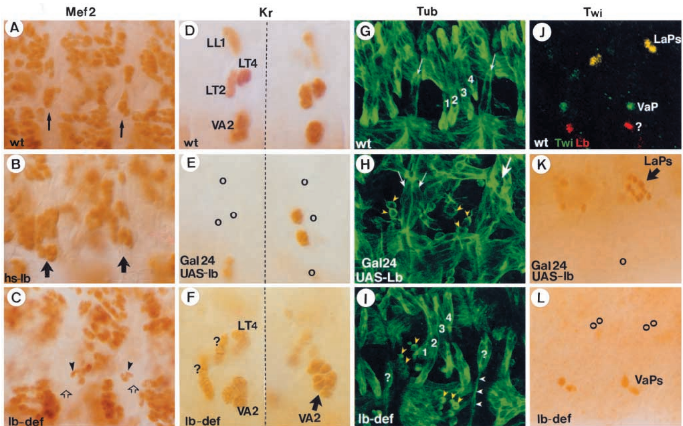
Fig. 5. lb determines the identity of both the SBM and LaPs. (A-C) Muscle pattern of the lateral part of abdominal segments immunostained with anti-Mef2. (A) Arrows point to SBMs of a wild-type embryo. (B) In hs-lb embryos, supernumerary myoblasts fuse to form enlarged SBMs (large arrows). (C) In embryos lacking lb activity, the SBMs are absent (open arrows). Arrowheads indicate some myoblasts lying near segmental borders. (D-F) Patterns of Kr -positive muscle precursors. (G-I) Confocal scans of muscle fiber architecture labeled with anti- \beta 3-Tub. (J-L) Patterns of lateral (LaP) and ventral (VaP) precursors of adult muscles: (J) double stained for twi (green) and lbe (red) or (K,L) detected with anti-Twi antibody. Note that, in J, the lb -positive SBM cells are not shown. Dotted lines (D-F) indicate the segmental borders. (D,G,J) Wild-type, (E,H,K) 24B-Gal4;UAS-lb and (F,I,L) lb -deficiency embryos. Ectopic lb expression in all mesodermal cells (E) changes the identity of the majority of Kr -positive muscle precursors (open circles) and (H) leads to the formation of duplicated (two arrows) or enlarged (large arrow) SBMs as well as to (K) the hypertrophic pattern of the LaPs (large arrow) and absence of the VaP (open circle). Yellow arrowheads in H point to unfused myoblasts lying within usual emplacement of lateral transverse muscles. In lb -deficiency embryos the lack of lb activity (F) leads to the formation of supernumerary (?) or enlarged (large arrow) Kr -expressing muscle precursors as well as to (L) the absence of LaPs (open circles) and duplication of VaP. (I) In lb -def embryos, the presence of unfused myoblasts around the normal SBM location (yellow arrowheads) and/or the formation of muscle fibers which lay within segmental borders but have abnormal shape (?) and insertion sites. This latter is illustrated by a muscle fiber (?) with a long filopodium (white arrowheads), most likely unable to recognise epidermal insertion site specific for the SBM. In all panels, anterior is to the left and dorsal is up. Abbreviations: 1,2,3,4, lateral transverse muscles LT1, 2, 3 and 4; LL1, lateral longitudinal muscle 1; VA2, ventral acute muscle 2.
