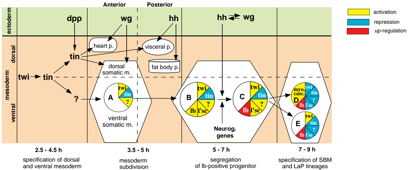
Fig. 7. Schematic representation of genetic events leading to the specification of SBM and LaP myoblast lineages. During gastrulation, mesodermal cells express twi , which activates tin in the region of the trunk. In the response to ectodermal Dpp signaling (Frasch, 1995), tin expression becomes restricted to the dorsal mesoderm suggesting that an unknown factor (?) specifies ventrally located mesodermal cells. Epidermal Wg and Hh signalings provide positional information leading to the mesoderm segmentation. Dorsal mesoderm located under the anterior, wg -expressing epidermal compartment gives rise to the heart and to the dorsal somatic muscles while the posteriorly located dorsal mesodermal cells (under the Hh influence) develop on visceral and fat body primordia (Azpiazu et al., 1996). In parallel, the ventral somatic muscles arise from the anteriorly located ventral mesodermal cells. Genetic events leading to the specification of two ventral somatic lineages: SBM founder and LaPs are illustrated in a series of circles, labelled A-E showing the activation or repression of gene activity. Multipotent ventral somatic mesodermal cells (A) differentiate to l'sc -expressing cells organized in promuscular clusters. In the case of the SBM promuscular cluster, these cells (B) start to express lb . Under the influence of epidermal signals and cell-cell signaling mediated by the neurogenic genes, the lb expression in the SBM progenitor (C) is upregulated. The SBM founder cell (D) continues to express lb and switches off twi activity while the LaPs (E) maintain both lb and twi expression. Since twi expression does not prevent differentiation of larval muscles (Baylies and Bate, 1996), its inactivation in the SBM founder, most likely, has no influence on the activation of the myogenic regulatory cascade. In contrast, according to Anant et al., 1998, persistent twi expression may keep, during embryonic and larval life, a nondifferentiated fate of adult muscle precursors.
