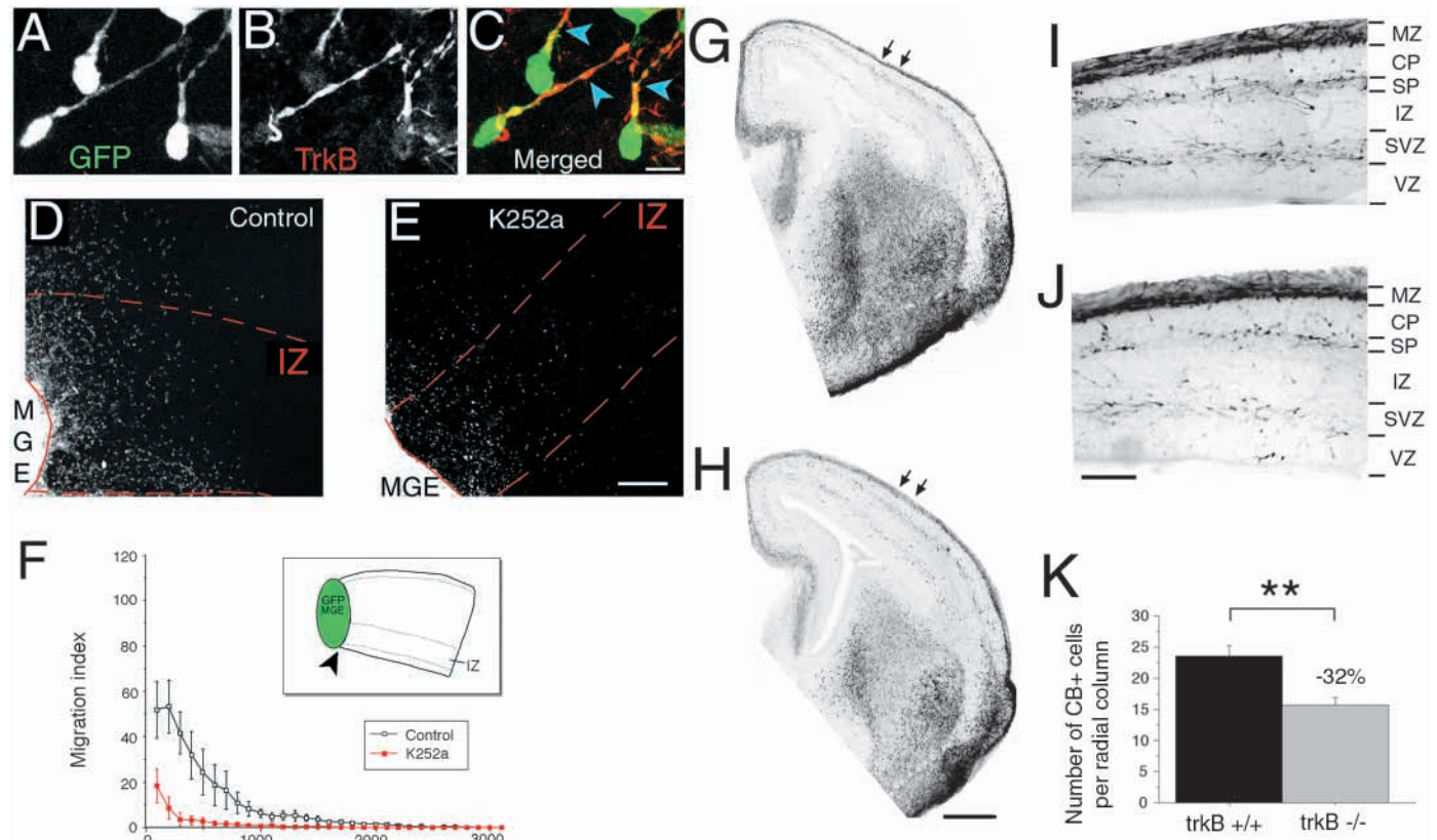
Fig. 7. Localization and function of TrkB receptors in tangential migration. (A-C) Double immunofluorescence for GFP (A) and TrkB (B) indicates that E14 MGE-GFP cells migrating in the cortical intermediate zone express the TrkB receptor (merged image in C). Note that the TrkB receptor is localized to the leading processes (arrowheads in C) of MGE-GFP cells. (D-E) Confocal images of E14 MGE-GFP cells migrating tangentially into the IZ of early postnatal cortex in the presence of control vehicle (DMSO 1:1000; D) or 50 nM of the Trk tyrosine kinase inhibitor K252a (E). (F) Quantification of the experiments shown in D,E from six slices taken from three independent experiments. Conventions are the same as in Fig. 6E. K252a treatment (red) significantly inhibits migration according to an ANOVA test ( F=28.53 ; P<0.0001 ). (G-H) Analysis of tangential migration in wild-type and TrkB null mice. (G-H) Low magnification photographs of coronal sections of E15 wild-type (G) and TrkB -/- mice (H) stained for calbindin 28K. At this rostrocaudal level of section, the global cytoarchitecture of the telencephalon in the two genotypes is indistinguishable. (I-J) High magnification photographs of the lateral cortex of sections shown in G,H. Tangentially migrating calbindin + cells are found mainly in the subventricular zone (SVZ), the upper part of the intermediate zone (IZ), the subplate (SP) as well as in the marginal zone (MZ) in both wild-type (I) and TrkB -/- (J) cortex. (K) Quantification of the number of calbindin + cells per 200 \mu\text{m} wide radial column (indicated by double arrows in G,H). This analysis reveals a significant decrease in the number of tangentially migrating calbindin + cells in TrkB -/- cortex compared with TrkB +/+ cortex at E15 [-32%; ** P<0.005 – Mann-Whitney test; 12 sections from three wild-type and three knockout mice]. Scale bars: 15 \mu\text{m} in A-C; 250 \mu\text{m} in D,E, 400 \mu\text{m} in G,H; 120 \mu\text{m} in I,J.
