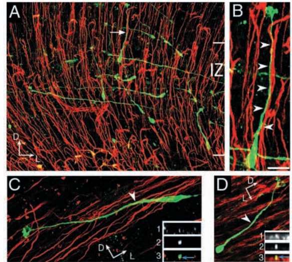
Fig. 4. Cellular interactions of MGE-derived tangentially migrating neurons. (A,B) Relationship between the leading process of E14 GE-GFP cells and the radial glial fibers in the intermediate zone (red, nestin). Cells migrating tangentially in the intermediate zone make several contacts with radial glial fibers, whereas some of the cells invading the cortical plate that migrate radially (arrow in A, shown at higher magnification in B) make multiple close contacts with the nestin+ glial fibers (arrowheads in B). In each image, the dorsal (D) and lateral (L) aspects are indicated. (C) Example of a migrating E14 GE-GFP cell making a few close contacts with axons (red, neurofilament 165 kDa) within the cortical intermediate zone. The insets numbered 1 (red, NF 165 kDa), 2 (green, GFP) and 3 (1 and 2 merged) represent a X-Z orthogonal section taken at the level indicated by the arrowhead in C. The blue arrows (3) indicate the location of close contact between an axon (red) and the leading process (green) of the tangentially migrating cell shown in C. (D) Example of an E14 GE-GFP cell migrating radially in the cortical plate towards the pia. This GE-GFP neuron makes contacts with cortical apical dendrites, revealed by MAP2 immunofluorescence (red). The insets numbered 1 (red, MAP 2), 2 (green, GFP) and 3 (1 and 2 merged) represent a X-Z orthogonal section taken at the level indicated by the arrowhead in D. The blue arrows (3) indicate the location of a close contact between an apical dendrite and the leading process of the GFP+ cell shown in D. Scale bars: 80 \mu\text{m} in A; 20 \mu\text{m} in B,C; 30 \mu\text{m} in D.
