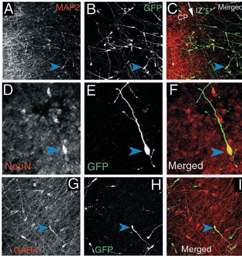
Fig. 3. Fate of MGE-derived tangentially migrating cells. (A-C) After 2 days in vitro, about 85% of E14 MGE-GFP cells (green, B) that migrate into the intermediate zone (IZ) express the neuronal marker MAP2 (A, red in C). The arrow in C delineates the border between the cortical plate (CP) and the IZ. (D-F) After 3 days in vitro, about 65% of E14 MGE-GFP cells (E, green in F) migrating in the IZ express the nuclear neuronal marker NeuN (D, red in F). (G-I) After 7 days in vitro, about 35% of E14 MGE-GFP cells (H, green in I) found in the cortex express the neurotransmitter GABA (G, red in I). Blue arrowheads indicate examples of double-labeled cells. Scale bars: 150 \mu\text{m} in A-C, G-I; 60 \mu\text{m} in D-F.
