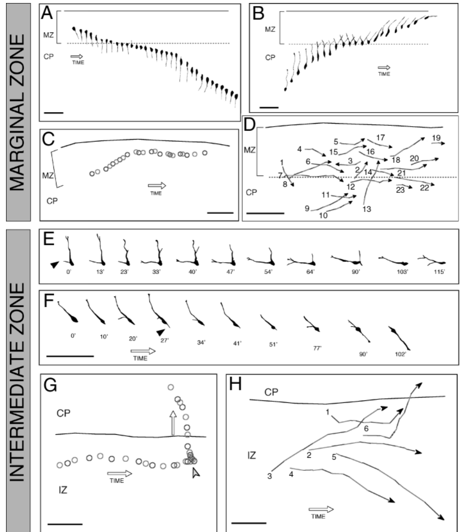
Fig. 5. Dynamics of tangentially migration MGE-GFP neurons. (A,B) Time-lapse analysis of MGE-GFP cells in isochronic co-cultures moving radially down from the MZ to the CP (A) and from the CP to the MZ (B). The position and morphology of the migrating cells is shown at 15 minute time intervals. Note that in each case, the cells pause at the interface between the MZ and the CP before crossing into the new zone. (C) Illustration of the kinetics of migration of an E15 GE-GFP cell within the MZ. Each circle represents the position of the cell body every 15 minutes and reveals that the cell body translocates according to a saltatory mode of migration. (D) Trajectories of 23 MGE-GFP cells migrating within the MZ. Twenty out of these 23 cells migrate coherently from the lateral (left-hand side) to medial (right-hand side) aspect of the cortex. One cell (#3) migrates mediolaterally, one cell (#1) migrates down into the CP and two cells (#13 and #2) migrate from the CP to the MZ. (E,F) Morphological dynamics of the leading process during a change in the direction of migration. These cells, migrating within the IZ, make 90° (E) or 180° (F) changes in their trajectory in less than 2 hours (time interval is indicated below each drawings). Note that in each case, the turn is not initiated by the growth cone of the leading process, but instead by a second leading process that emerges from the cell body. (G) Example of an MGE-GFP cells crossing from the IZ to the CP. Note that the cell initially migrating in the IZ pauses for a prolonged period (arrowhead) before changing its trajectory by 90° and entering the CP. The arrows indicate the direction of migration. Conventions as in C. (H) Trajectories of six GE-GFP cells migrating within the IZ. Note that most cells migrate from a lateral (left) to medial (right) direction. One cell can be seen changing trajectories to enter the CP. Scale bar: 50 \mu m in A-D,G-H; 100 \mu m in E,F.
