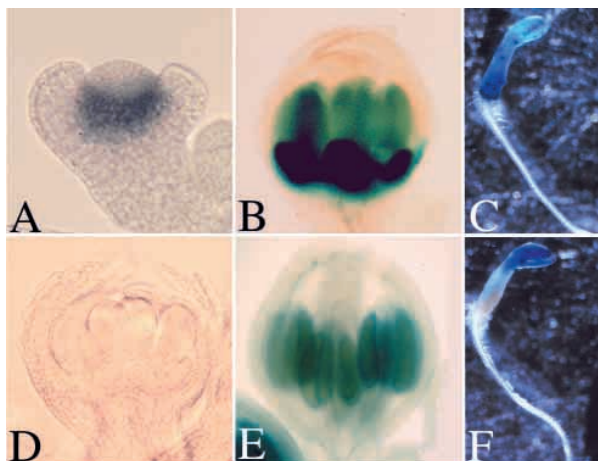
Fig. 5. Mutation of the LFY binding site in the AP3 promoter does not disrupt expression in planta. The 5D3::GUS construct containing site Im and site IIIm mutations ( 5D3-ImIIIm::GUS ) confers GUS expression in the presumptive petal and stamen primordia in a wild-type background both at stage 3 (A) and at stage 8 (B), similar to that seen for the unmutated version of 5D3::GUS (Hill et al., 1998). 5D3-ImIIIm::GUS also confers GUS activity in 35S::LFY , 35S::UFO seedlings (C). Expression of the D3-18 construct containing site Im and site IIIm mutations ( D3-18-ImIIIm ) in a wild-type background at stage 6 (D) and stage 10 (E). This pattern of GUS expression recapitulates that conferred by the unmutated D3-18::GUS construct (Hill et al., 1998). Furthermore, D3-18-ImIIIm::GUS is expressed in seedlings containing the 35S::LFY , 35S::UFO transgenes (F).
