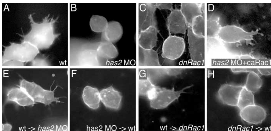
Fig. 5. Has2 and Rac1 act in a cell autonomous fashion, promoting lamellipodia formation. All panels show individual lateral mesodermal cells at the 80% epiboly stage, visualized with membrane-localized GFP. Dorsal is to the right, anterior to the top. (A) Wild type; (B) has2 morphant; (C) wild type injected with mRNA encoding dominant-negative Rac1 ( dnRac1 ); (D) has2 morphant injected with mRNA encoding constitutively active Rac1 ( caRac1 ); (E) wild-type cells transplanted into has2 morphant host; (F) has2 morphant cells transplanted into wild-type host; (G) wild-type cells transplanted into host expressing dnRac1 ; (H) dnRac1 -expressing cells transplanted into wild-type host.
