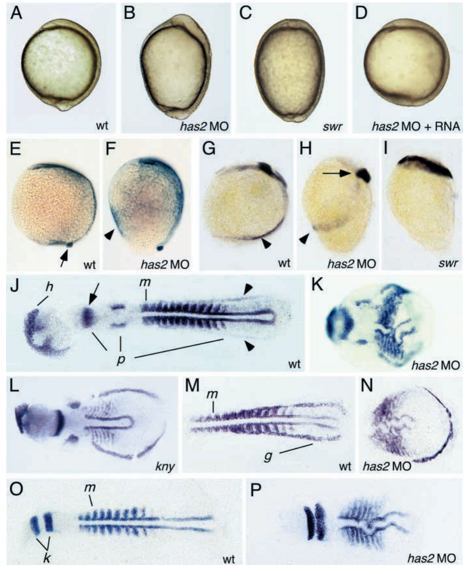
Fig. 3. has2 morphants are elongated, similar to Bmp mutants, but are not dorsalized. (A-D) Live embryos at tailbud stage, lateral view, dorsal to the right. (A) Wild type; (B) has2 morphant; (C) bmp2b/swr mutant; (D) embryo co-injected with has2 MO and has2 mRNA. (E,F) sox17 expression at tailbud stage, lateral views, dorsal to the right. (E) Wild type; (F) has2 morphant. Arrow (E) indicates forerunner cells; arrowhead (F) endodermal cells that have remained on the ventral side. (G-I) pax2.1 expression at the 4-somite stage, lateral view. Arrow (H) indicates midbrain-hindbrain boundary; arrowheads (G,H) indicate presumptive pronephric duct cells. (G) Wild type; (H) has2 morphant; (I) swr mutant. (J-L) pax2.1 (marked as 'p'), myoD ('m'), hgg1 ('h') expression at the 10-somite stage; dorsal views on regular (K) or flat-mounted (J,L) embryos. (J) Wild type; (K) has2 morphant; (L) kny/glypican6 mutant. In J, midbrain-hindbrain boundary is marked by an arrow, pronephric ducts by arrowheads. (M,N) gata1 ('g') and myoD ('m') expression at the 10-somite stage; dorsal view on flat-mounted embryos. (M) Wild type; (N) has2 morphant. (O,P) krox20 ('k') and myoD ('m') expression at the 10-somite stage; dorsal view on flat-mounted embryos. (O) Wild type; (P) has2 morphant.
