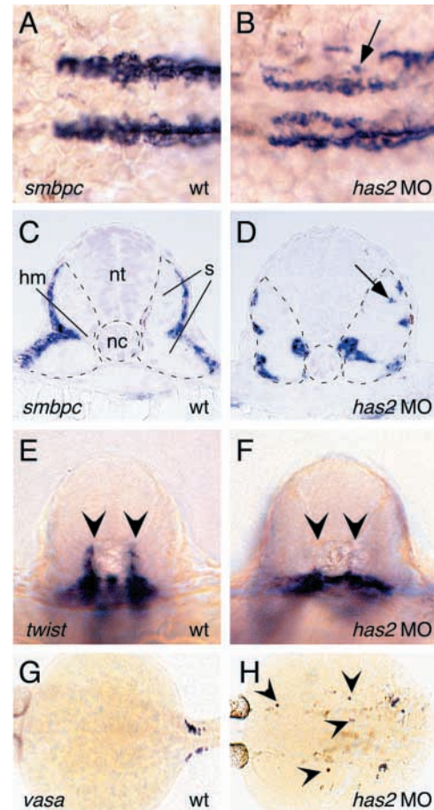
Fig. 7. Has2 is required for migration of presumptive slow muscle and sclerotomal cells during morphogenesis of somites, and for the migration of primordial germ cells. (A-D) 30 hpf; smbpc in situ hybridization to mark slow muscle cells of trunk somites: (A,C) wild type; (B,D) has2 morphant. (A,B) Dorsal view, anterior left; (C,D) transverse sections. Arrows (B,D) mark smbpc -positive cells located within the presumptive fast muscle tissue. The lower side of the embryo in B is less affected, which might have been the reason for its survival. The effects are restricted to the first 5-8 somites, consistent with previous findings indicating different properties between such anterior and more posterior somites (see van Eeden et al., 1996). (E,F) twist in situ hybridization, at 24 hpf, to mark sclerotomal cells of trunk somites. Arrowheads indicate dorsally migrated sclerotomal cells in wild type (E), which remain ventral in has2 morphant embryos (F). (G,H) Distribution of vasa -positive primordial germ cells, at 24 hpf, in wild type (G) and has2 morphant (H). Arrowheads (H) point to ectopic PGCs outside the genital ridges. hm, horizontal myoseptum; nc, notochord; nt, neural tube; s, somite.
