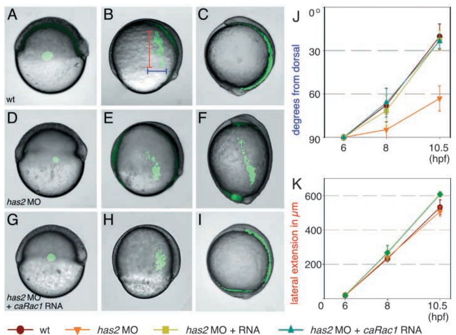
Fig. 4. Loss of Has2 function leads to blockage of dorsal convergence, but not of extension, and can be compensated by constitutively active Rac1.
