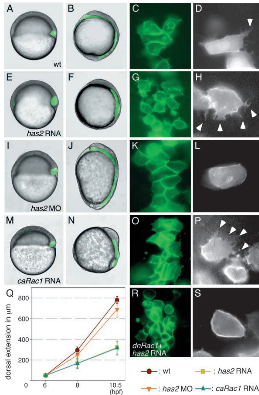
Fig. 6. Forced dorsal expression of has2 and constitutively active Rac1 lead to supernumerary lamellipodia, blocking axis extension. Extension movement of labeled populations of dorsal cells. (A-D) Wild-type control embryos; (E-H) embryos injected with has2 mRNA; (I-L) has2 morphant embryos; (M-P) embryos injected with caRac1 RNA; (R,S) embryos co-injected with has2 mRNA and dnRac1 mRNA. The first two columns show uncaging experiments. Lateral view of embryos at shield stage (6 hpf), directly after uncaging (A,E,I,M), or at tailbud stage (10.5 hpf; B,F,J,N). Columns 3 and 4 show morphology of clusters (C,G,K,O,R) or individual (D,H,L,P,S) dorsal cells labeled with membrane-localized GFP. Arrowhead (D) indicates single lamellipodium sometimes visible on narrow dorsal side of highly polarized axial cells of wild-type embryos. Arrowheads (H,P) indicate multiple lamellipodia in axial cells of has2 RNA- or caRac1 mRNA-injected embryos. (Q) Graph showing the amount of extension in the axis of wild-type, has2 MO-, has2 mRNA- or caRac1 mRNA-injected embryos. Per treatment, ten different embryos were evaluated, and standard deviations are indicated.
