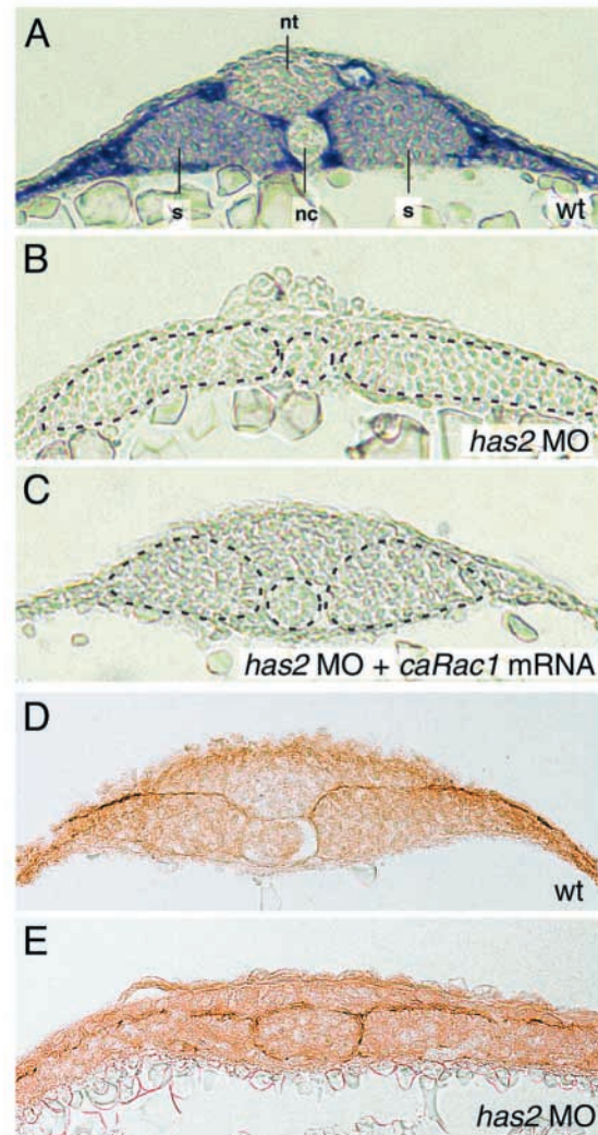
Fig. 2. Presence of HA depends on Has2 activity and cannot be restored by constitutively active Rac1, whereas Fibronectin is unaffected in has2 morphants. (A–C) HA staining on transverse sections through the posterior region of 10-somite stage embryos. (A) Wild type; (B) embryo injected with has2 MO; (C) embryo co-injected with has2 MO and mRNA encoding constitutively active Rac1 ( caRac1 ). At tailbud stage, the embryo in C was elongated, indicating convergence defects, the embryo in B was round like the wild-type control, indicating that convergence was rescued (compare with Fig. 4). Notochord and somites are outlined in B,C. (D,E) Anti-Fibronectin immunostaining. Section through posterior region of 3-somite stage embryos. (D) Wild type; (E) embryo injected with has2 MO. nc, notochord; nt, neural tube; s, somite.
