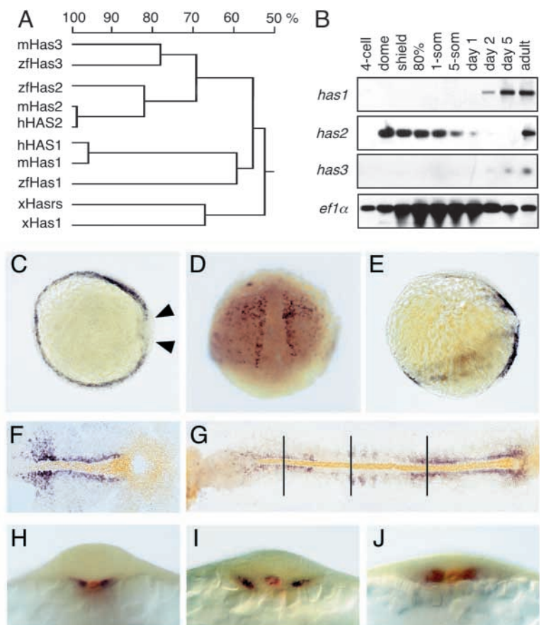
Fig. 1. Zebrafish Has genes and their expression during embryogenesis. (A) Homology tree of Has1, Has2, and Has3 family members based on amino acid sequences. The GenBank accession numbers for the sequences listed above are: Xenopus laevis xHas1 (X52958), Xenopus laevis xHasrs (AF015780), mouse mHas3 (MMU86408), human hHAS2 (HSU54804), mouse mHas2 (MMU52524), human hHAS1 (HSU59269), mouse mHas1 (D82964). (B) RT-PCR analysis of zebrafish has1 , has2 and has3 expression during different stages of development. (C-J) Wild-type embryos stained for has2 mRNA (blue), and No tail (Ntl) protein (brown; F-J). (C) Early gastrulation (shield stage), animal pole view. Arrowheads indicate the dorsal shield devoid of staining. (D) Midgastrulation (80% epiboly stage), dorsal view. (E) 90% epiboly stage, lateral view, dorsal to the right. (F) End of gastrulation (100% epiboly stage), dorsal view on flat-mounted embryo; anterior to the left. (G-J) 8-somite stage: (G) dorsal view on flat-mounted embryo, anterior to the left; (H-J) optical cross sections at levels indicated in G.
