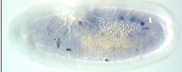
D tin-/-; lbl intronic-LacZ
