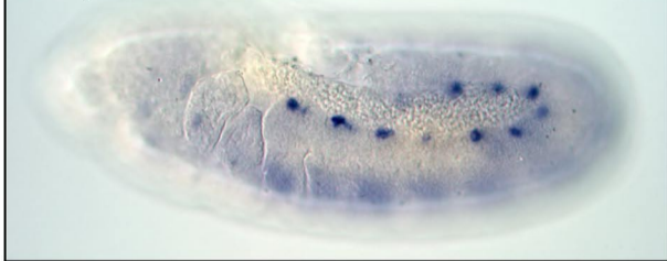
A wt; lbl downstream-LacZ
