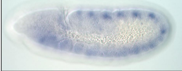
B tin-/-; lbl downstream-LacZ
