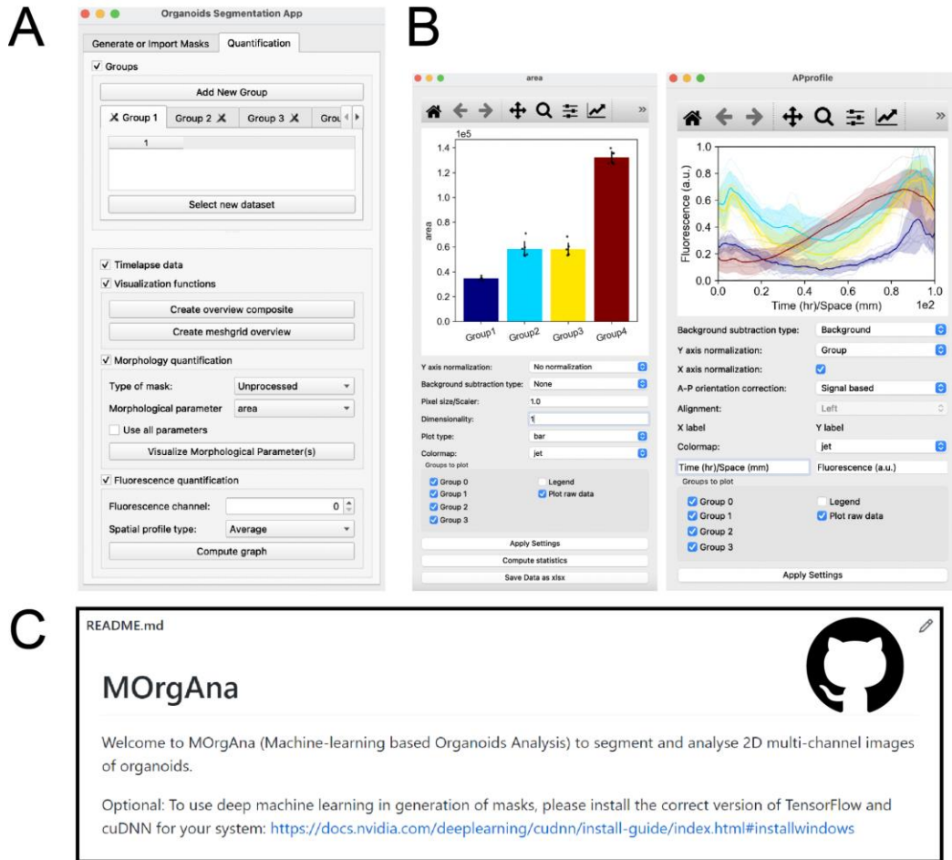
Supplementary Figure 2: Graphical user interface of MORGAna and GitHub page: quantification and output. A) Panel to cluster different datasets into separate “groups” for future visualization and comparison. Datasets can be treated as time lapse (tick box). Overview images can be generated with the “Visualization functions” buttons. B) Morphology (left) and Fluorescence intensity (right) visualization graphs can be generated and datasets from different groups easily compared. C) The GitHub repository at which all open-source MORGAna code is found. In the same repository, advanced users can find ready-to-use Jupyter Notebooks.
