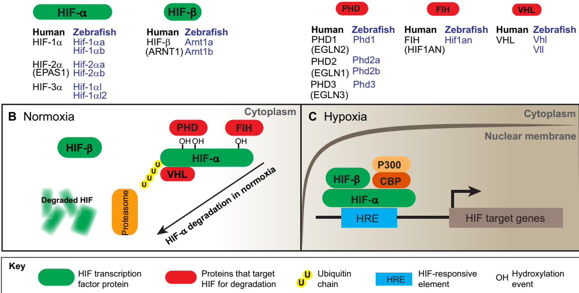
Fig. 1. Schematic diagram of the HIF-signalling system and zebrafish homologues. (A) Proteins of the HIF-signalling pathway are illustrated, with HIF proteins in green and proteins that target HIF for degradation in red. The human isoforms are listed, with their zebrafish counterparts in blue text. (B) In normoxia, the hydroxylase enzyme PHD and the VHL protein target HIF- \alpha for ubiquitination in the cytoplasm and subsequent degradation by the proteasome. A second hydroxylase enzyme, FIH, hydroxylates a C-terminal asparagine residue on HIF- \alpha in normoxia to repress the transactivation function of HIF. (C) In hypoxia, hydroxylase enzymes are silenced, and HIF translocates to the nucleus and binds its cofactors, where it upregulates target gene expression by binding to HREs in their regulatory regions. Abbreviations: CBP, CREB-binding protein; FIH, factor inhibiting HIF; HIF, hypoxia-inducible factor; HREs, HIF-responsive elements; P300, E1A binding protein; PHD, prolyl hydroxylase domain-containing proteins; VHL, von Hippel-Lindau.
