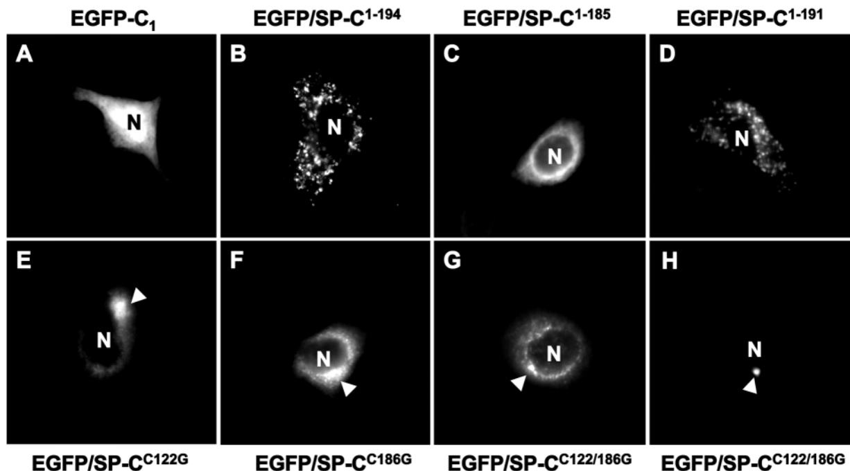
Fig. 2. C-mutants lacking Cys 186 and/or Cys 122 are retained in proximal compartments. A549 cells were transiently singly transfected either with EGFP-C 1 (A), EGFP-C 1 /SP-C 1-194 (B), the C-truncation mutants EGFP-C 1 /SP-C 1-185 (C) and EGFP-C 1 /SP-C 1-191 (D), or the C-cysteine mutants EGFP-C 1 /SP-C C122G (E), EGFP-C 1 /SP-C C186G (F) and EGFP-C 1 /SP-C C122,186G (G,H), using CaPO 4 . Images for EGFP expression were acquired 48 hours after transfection by fluorescence microscopy with a High Q fluorescein isothiocyanate (FITC) filter package (excitation at 480 nm, emission at 535/550 nm). Expression of EGFP-C 1 /SP-C 1-194 as well as EGFP-C 1 /SP-C 1-191 was in cytoplasmic vesicles. In contrast, EGFP-C 1 /SP-C 1-185 is translocated but failed to reach cytoplasmic vesicles. As with EGFP-C 1 /SP-C 1-185 , all three cysteine mutants (E-H) were restricted to a juxtannuclear region and showed variable degrees of aggregation (arrowheads).
