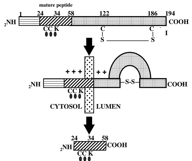
Fig. 1. Biosynthesis of SP-C. Rat SP-C is synthesized by the alveolar type 2 cells as a proprotein of 194 aa (SP-C 21 ). Contained within the propeptide is the 35-aa mature SP-C protein (SP-C 3,7 ), which is flanked by propeptides of 23 amino acids at the N terminus and 136 residues at the C terminus. After translation, SP-C 21 is translocated to the endoplasmic reticulum (ER) and inserted into the ER membrane as a bitopic protein in a type II membrane orientation, which is anchored by the \alpha -helical domain Leu 36 -Leu 55 contained within the mature SP-C sequence. The proSP-C C terminus contains conserved cysteine residues, which could participate in disulfide-mediated folding in the oxidizing environment of the ER lumen. Proteolytic removal of the C- and N-flanking domains is Brefeldin A-sensitive, indicating that processing is dependent upon delivery of SP-C 21 to post-Golgi processing compartments. Within the mature peptide, aa residues Cys 28 , Cys 29 , and Lys 34 (CCK) have been shown to contain covalent palmitic acid.
