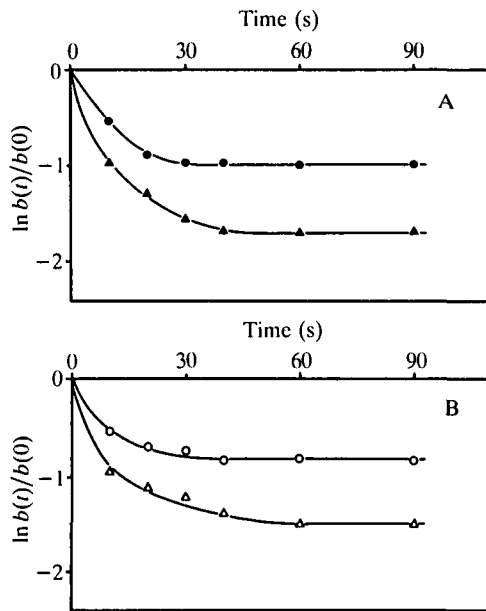
Fig. 5. Semi-logarithmic plot of dissociation of 100 nM- ^3\text{H} GTP from membranes. Wild-type (A) and mutant (B) membranes were preincubated for 90 s with 100 nM- ^3\text{H} GTP; then, at t = 0 rapidly mixed with 0.1 mM-GTP (●, ○) or 0.1 mM-GTP and 10 \mu\text{M} -cyclic AMP (▲, △). The results are the means of three experiments, with the standard error less than 10% of the mean.
