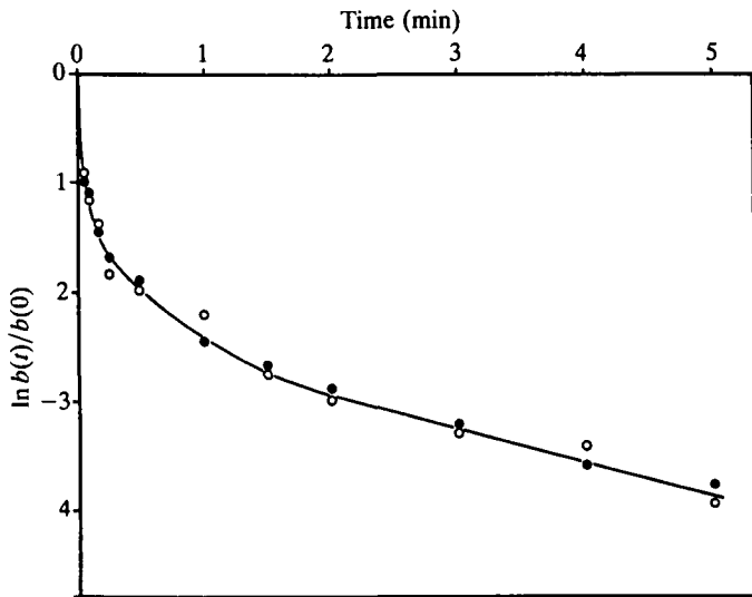
Fig. 2. Dissociation kinetics of [ 3 H]cyclic AMP-receptor complex. Wild-type (●) and mutant cells (○) were preincubated with 2 nM-[ 3 H]cyclic AMP for 45 s, and dissociation was induced at t = 0 by the addition of 0.1 mM-cyclic AMP. Binding was detected at the times indicated, b(0) and b(t) . The means of two experiments are presented.
