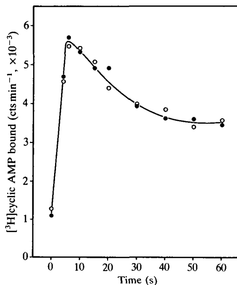
Fig. 1. Association of 30 nM- ^3\text{H} -cyclic AMP to wild-type (●) and synag 7 mutant cells (○). Cells were incubated at 20°C with cyclic AMP and total cyclic AMP binding was measured at the times indicated. The results shown are the means of two experiments in triplicate, with intra-assay variation of less than 4% of the means.
