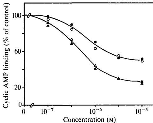
Fig. 3. Inhibition of the binding of 2 nM-[ 3 H]cyclic AMP to wild-type (●, ▲) and mutant (○, △) membranes by GDPβS (●, ○) and GTPγS (▲, △) after an incubation period of 75 s. The means of four experiments are shown with the error less than 10% of the means.
