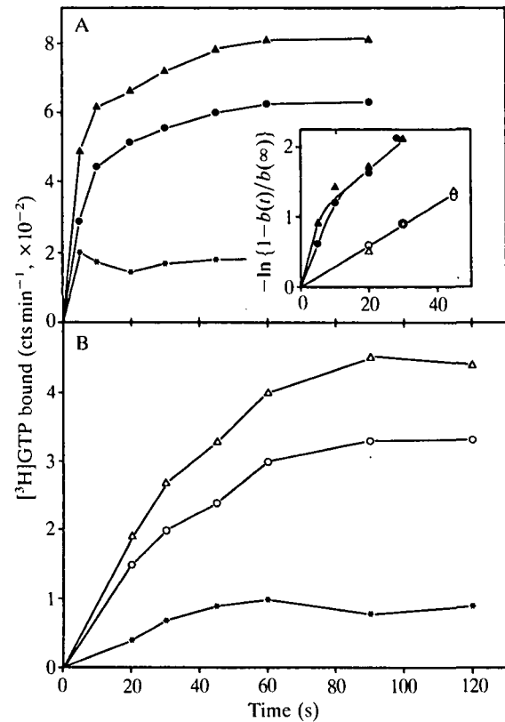
Fig. 4. Association of 100 nM-[ 3 H]GTP to wild-type (A) and mutant (B) membranes in the absence (●, ○) or presence (▲, △) of 10 μM-cyclic AMP. The results shown are the means of three experiments in triplicate, with intra-assay variation of less than 3%. Inset: b_{\infty} equals the specific binding at equilibrium (90 s), b_t at t . The means of three experiments are presented, with the standard error less than 10% of the means. The asterisks represent differences between (▲, △) and (●, ○).
