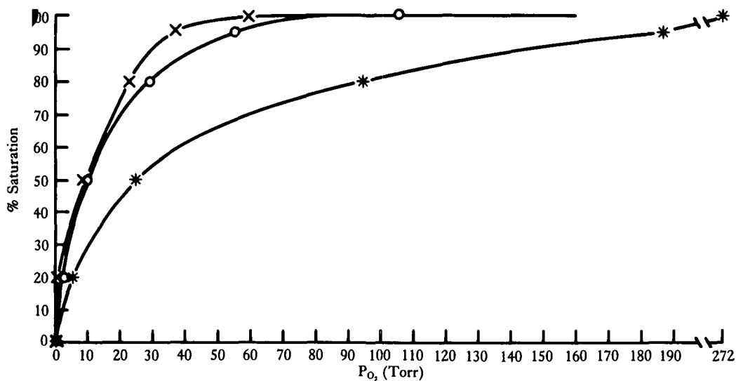
Fig. 3. Whole blood oxygen dissociation curves from albacore ( Thunnus alalunga ) no. 5, equilibrated at 0% \text{CO}_2 and 25°C (O), and at 10°C and then quickly warmed to 30°C (×), and at 1% \text{CO}_2 and 30°C and then quickly cooled to 10°C (*).
