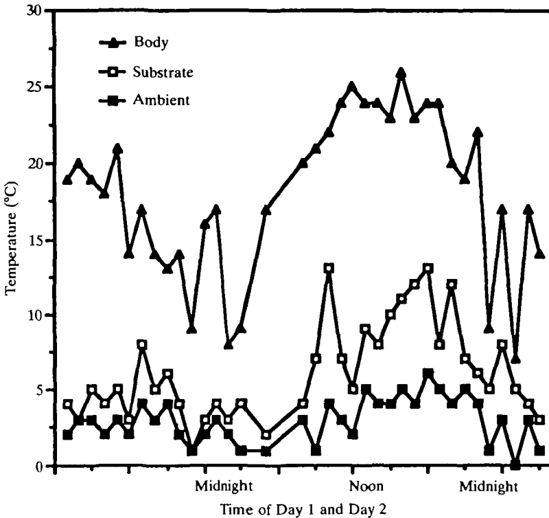
Fig. 3. Diel changes in mean body temperature ( \pm s.d. \leq 5 ) of eight Gynaephora groenlandica larvae relative to ambient and substrate temperatures recorded approximately bihourly over 2 days (an overcast day followed by a sunny one) on the open tundra.
