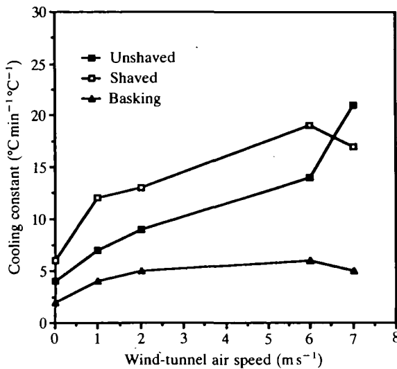
Fig. 4. Influence of increasing wind velocity on the cooling constants (see text for explanation) of unshaved, shaved and basking larvae of Gynaephora groenlandica ( N = 3 , \pm s.d. \leq 1.5 ).
