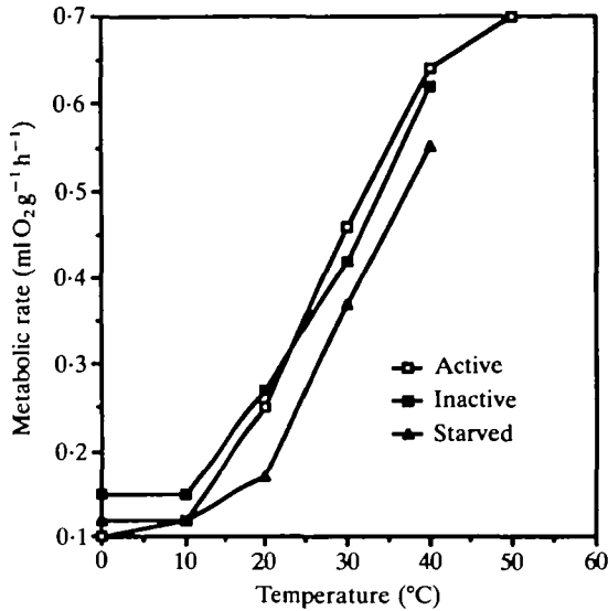
Fig. 6. Metabolic rate as a function of body temperature (range from 0 to 50°C) recorded for 10 actively feeding, active but starved and inactive larvae of Gynaephora groenlandica ( \pm s.d. \leq 0.03 ).
