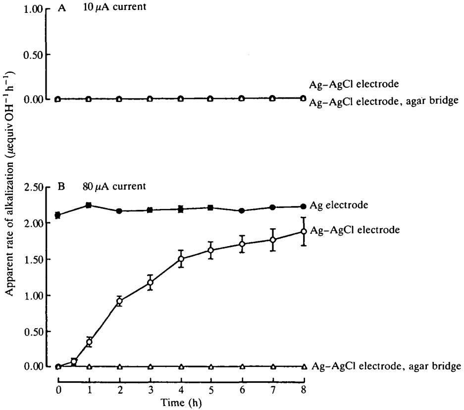
Fig. 2. Effect of electrode configuration and quantity of current passed on apparent rates of luminal alkalization. (A,B) 10 or 80 \mu\text{A} of current passed across the current-sending electrodes, respectively. Experimental chambers were set up without recta and filled with the standard \text{CO}_2/\text{HCO}_3^- -free saline used throughout this study. Rates of alkalization were measured by pH-stat (saline pH maintained at 7.00). Values are means \pm s.e. (where larger than symbol); N=6 .
