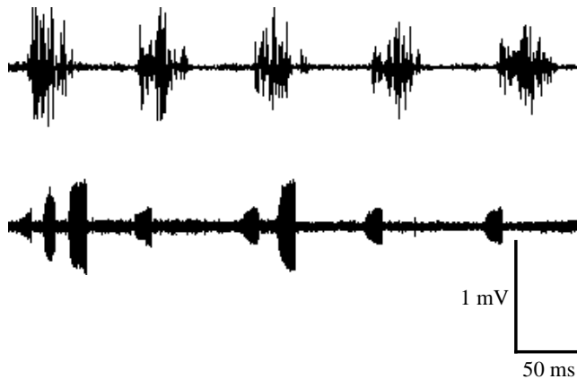
Fig. 18. Activity of the serratus ventralis (upper trace) in relation to biosonar vocalization (lower trace) in a flying bat. The amplitude scale applies only to the electromyogram.
