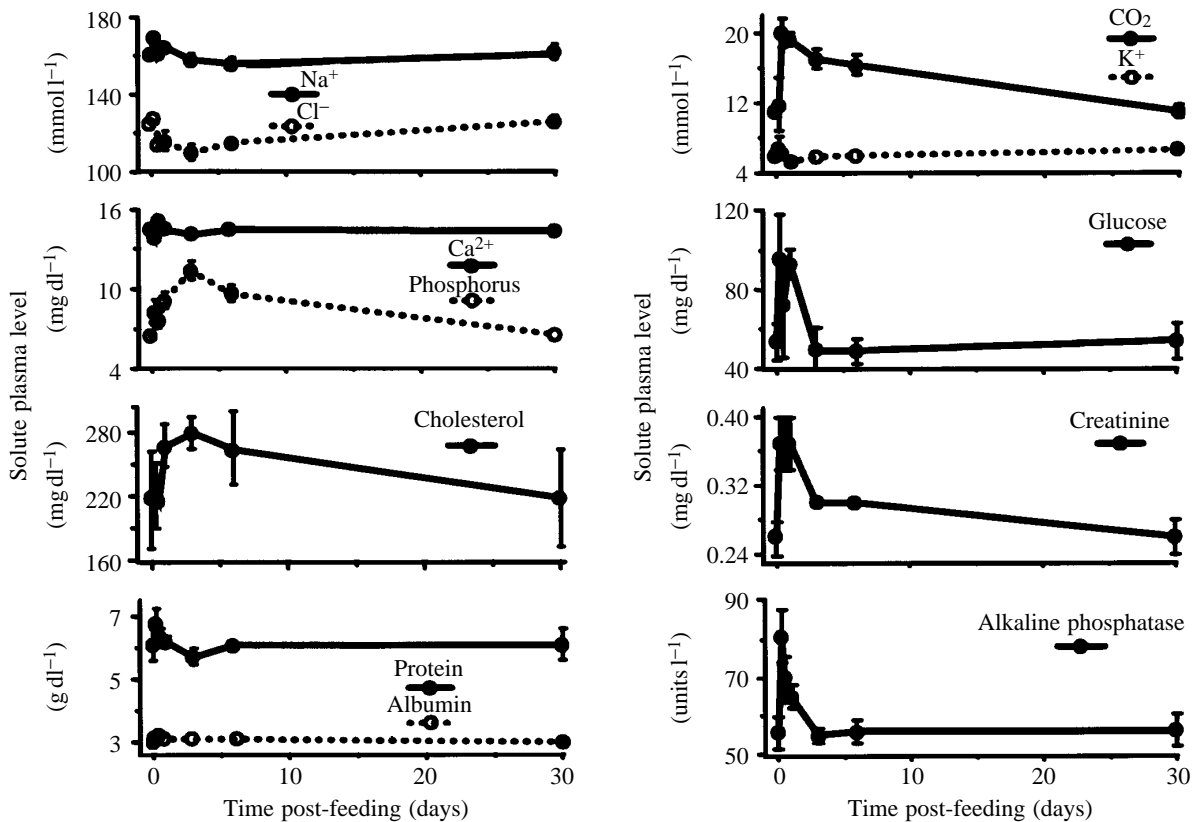
Fig. 7. Solute plasma levels, as a function of days post-feeding. Note the post-feeding decrease in Cl^- and rises in CO_2 , phosphorus, creatinine and alkaline phosphatase levels. Alkaline phosphatase activity is measured in international units.
