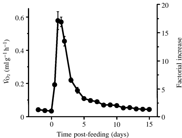
Fig. 1. Mean \text{O}_2 consumption rates of Burmese pythons ( N=8 ) for 3 days before and 15 days after consuming a rat meal equivalent in mass to approximately 25% of the snake's body mass. The right-hand axis shows the factorial increases in \dot{V}_{\text{O}_2} above pre-feeding values. In this and subsequent figures, vertical bars represent \pm 1 S.E.M. or least-squares mean, but bars are omitted if they are smaller than the symbol for the mean value. Note that \dot{V}_{\text{O}_2} peaks at day 1 post-feeding, at a value 17 times that before feeding.
