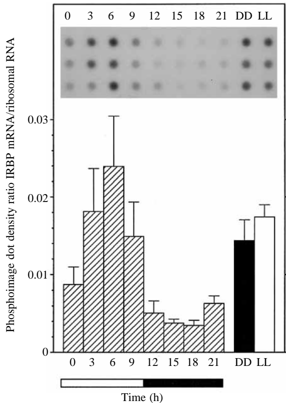
Fig. 9. IRBP mRNA expression under cyclic and constant conditions. Zebrafish were entrained under a 12h:12h L:D (06:30h lights on/06:30h lights off, LD) cycle and were killed at 3h intervals beginning at light onset. Other zebrafish, maintained for 8 days in constant dark (DD) or constant light (LL), were killed at subjective noon. For each time point and constant condition, six pairs of eyes were separately extracted and dotted. The ratio of [ ^{32} P]IRBP cDNA hybridization to that of each dot reprobod with a [ ^{32} P]18S ribosomal RNA cDNA is compared in each experimental condition. The inset is a representative autoradiogram of dots probed with the IRBP cDNA. Bar under graph: open, light; filled, dark. Error bars are standard errors of the mean, N=6 .
