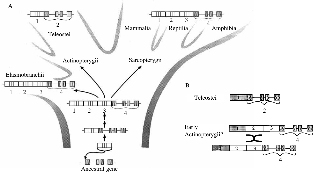
Fig. 11. Model of the evolution of IRBP. (A) IRBP probably arose from an ancestral gene through insertion of a processed gene followed by two unequal crossover events (Borst et al. 1989). Mammals, reptiles, amphibians and possibly Elasmobranchii (IRBPs from sharks, skates and rays have not been cloned) have such a four-module IRBP. At some point during the evolution of the Actinopterygii (which gave rise to modern teleosts), the middle two modules of IRBP were lost. (B) On the basis of the observation that the first and last repeats of zebrafish and human IRBPs are the most similar, we envision that during the evolution of the ray-finned fish (Actinopterygii) the middle two modules were lost from an ancestral four-module IRBP through an unequal crossover event.
