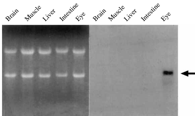
Fig. 2. Tissue distribution of the mRNA for IRBP. Left: ethidium-bromide-stained agarose gel showing the ribosomal RNA subunits. Right: autoradiogram of the northern blot of the same gel. The blot was probed with the zebrafish IRBP cDNA labeled with ^{32}\text{P} . The mRNA for zebrafish IRBP is approximately 2.3 kb in size (arrow). 9 \mu\text{g} of total RNA was loaded on each lane from brain, muscle, liver, intestine and eye. The Kodak XAR film was exposed at -80^\circ\text{C} for 51 h with an intensifier screen.
