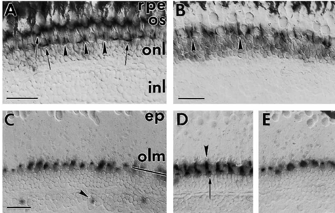
Fig. 8. In situ hybridizations of zebrafish IRBP and goldfish opsin cRNAs in zebrafish retinal cryosections. (A) Retina obtained at mid-light, hybridized with zebrafish IRBP cRNA. The reaction product is found in cone photoreceptor inner segment myoids (some examples are indicated by arrows), with weaker labeling of the perinuclear regions of rod photoreceptors in the outer nuclear layer (onl) and the rod myoids (some examples are indicated by arrowheads; compare with B). In this light-adapted retina, heavily pigmented processes of retinal pigmented epithelium (rpe) closely appose most of the cone outer and inner segments (os), but do not contact the outer segments of the short single (ultraviolet) cones, positioned immediately apical to the onl. inl, inner nuclear layer; scale bar, 25 \mu\text{m} . (B) Retina obtained at mid-light, hybridized with goldfish rod opsin cRNA. Reaction product is restricted to the rod perinuclear region and the rod myoids (two examples are indicated by arrowheads). Labeled rod myoids typically appear as narrow vertical bands of reaction product between the cone inner segments. Scale bar, 25 \mu\text{m} . (C) Retina obtained at mid-dark, hybridized with zebrafish IRBP cRNA. Reaction product is found only in one cone photoreceptor type; these cones have nuclei positioned within the outer limiting membrane (olm, delineated by the oblique line segment). In this dark-adapted retina, the retinal pigmented epithelial pigment has migrated basally (and does not appear in this photograph) and cone photoreceptors have elongated such that their outer segments are a substantial distance (50–80 \mu\text{m} ) from the corresponding cone nuclei and are not in view. The bases of the refractile inner segment ellipsoids (ep) are seen at the top. Rare inner nuclear layer neurons also hybridize with zebrafish IRBP cRNA (indicated by an arrowhead). Scale bar (applies to C, D and E), 25 \mu\text{m} . (D) Retina obtained at mid-dark, hybridized with a combination of zebrafish IRBP cRNA and goldfish blue cone opsin cRNA. Two distinct populations of cone photoreceptors show reaction product in their inner segments (arrow and arrowhead each indicate a member of one of these cone populations). (E) Retina obtained at mid-dark, hybridized with a combination of zebrafish IRBP cRNA and goldfish ultraviolet cone opsin cRNA. Only one population of cones has hybridized and the pattern matches that of the IRBP cRNA alone (compare with C).
