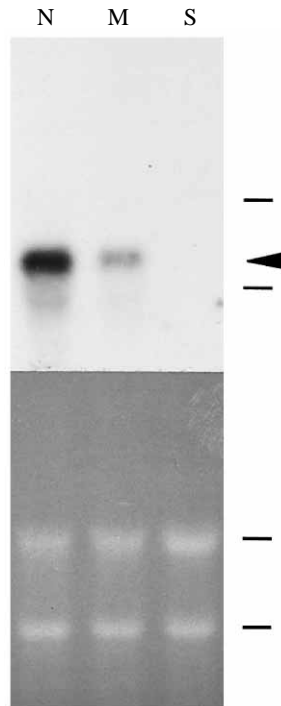
Fig. 6. Northern analysis of IRBP at noon (N) and midnight (M) under cyclic light. Top: autoradiogram of transfer, probed with ^{32}\text{P} -labeled full-length zebrafish IRBP cDNA ZF9. On the basis of the phosphoimage analysis, the radioactivity of the IRBP band (arrowhead) at noon is four times greater than at midnight. Bottom: ethidium-bromide-stained agarose gel (1% Seakem) showing the ribosomal subunits (dashes). 7\ \mu\text{g} of total RNA was loaded in each lane. Lane S corresponds to skeletal muscle (negative control). The Kodak X-AR film was exposed for 20h with an intensifier screen at -80^\circ\text{C} .
