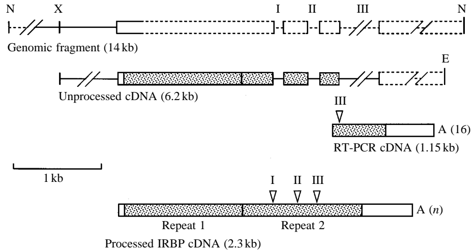
Fig. 1. Zebrafish genomic and cDNA clones. The upper three diagrams represent the cDNA and genomic clones isolated in the present study. The diagram at the bottom is the deduced 2.3 kb mRNA which consists of two modules. Arrowheads locate intron splice sites (I, II, III), which are restricted to the second module. Rectangles are exons; stippled regions are the coding sequences; dashed portions are unsequenced areas. Restriction enzymes: N, NotI ; E, EcoRI ; X, XhoI . A, poly(A) tail.
