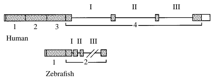
Fig. 4. Comparison of human and zebrafish gene structures. Both genes consist of homologous modules (four in human; two in zebrafish) of approximately 300 amino acids in length. In both species, the introns (I–III) are located at the same relative positions, splitting the last repeat. The first two introns are smaller in zebrafish. The last zebrafish intron is under study (interrupted line).
