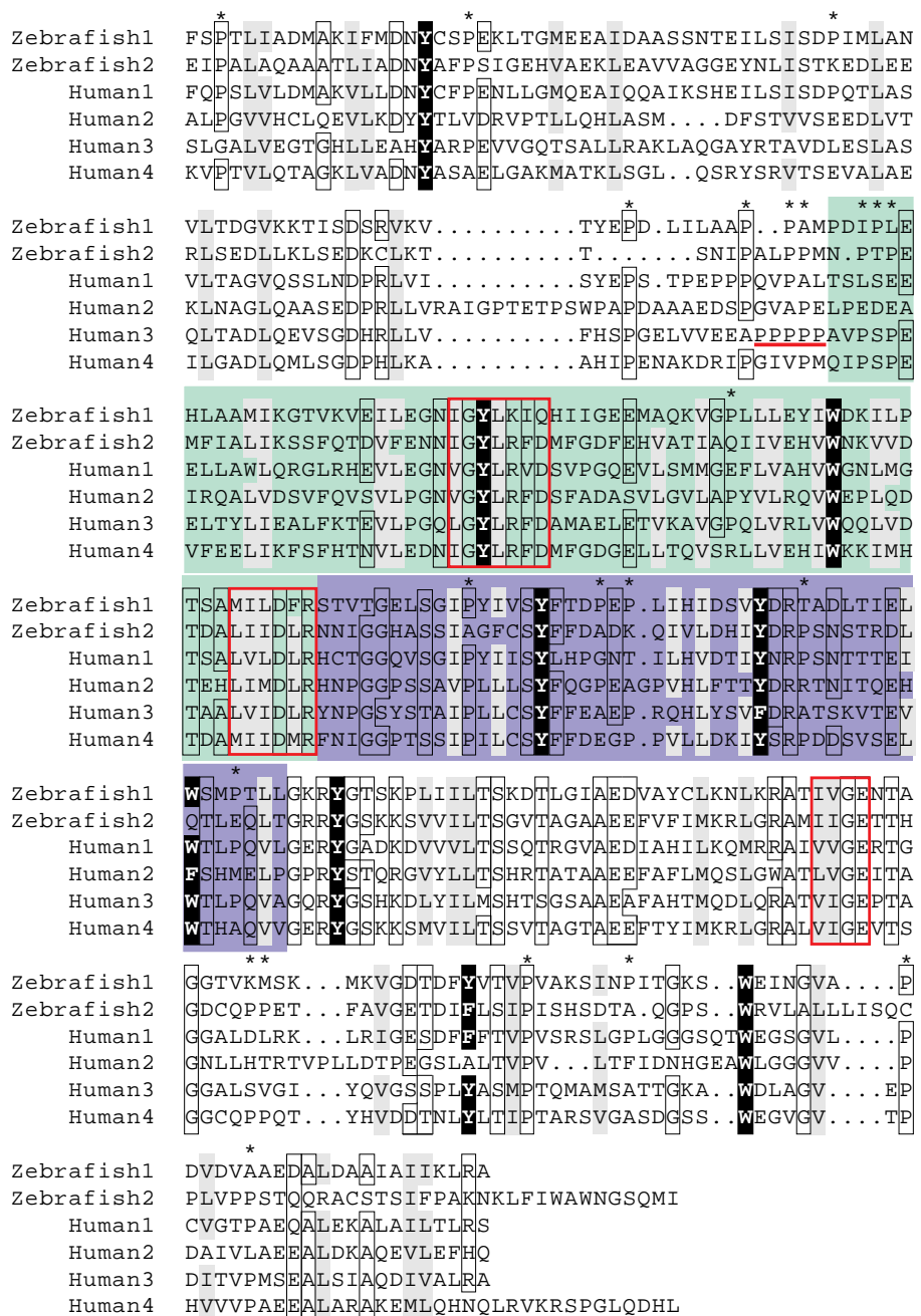
Fig. 5. Alignment of zebrafish and human IRBPs. The boundaries between the two modules of zebrafish IRBP and the four modules of human IRBP were determined using the program LALIGN. All the modules of both proteins were aligned using the program PILEUP (Wisconsin Genetic Package, GCG). Sequences corresponding to the second and third exons are highlighted in green and purple, respectively. Highly conserved regions are boxed in red (see text). A stretch of five consecutive prolines in the approximate center of human IRBP (at the beginning of the third module) is underlined in red. Prolines that are present at the same position in one zebrafish and one human module are marked with an asterisk. Chemically similar residues are indicated when five of the six were similar or identical: F=W=Y (black); I=L=V=M (gray); D=E=N=Q, S=T, A=G and R=K=H (boxed).
