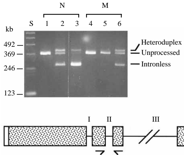
Fig. 7. RT-PCR analysis comparing unprocessed and intronless zebrafish IRBP mRNAs at noon (N) and midnight (M). Total ocular RNA was reverse-transcribed using random hexamers followed by amplification with PCR using primers flanking intron II. The presence or absence of this intron in the amplified message was confirmed by probing the Southern blot analysis of this gel with a labeled intron II oligomer. Lanes 1, 2 and 3 were transcribed from total ocular RNA taken from zebrafish killed at noon; and lanes 4, 5 and 6 were transcribed from total ocular RNA taken from zebrafish killed at midnight. The [\text{MgCl}_2] was 1.25\ \text{mmol l}^{-1} (lanes 1 and 4), 3.13\ \text{mmol l}^{-1} (lanes 2 and 5) and 5\ \text{mmol l}^{-1} (lanes 3 and 6). At the bottom is a diagram of the zebrafish IRBP gene. Under the gene diagram, the locations of the PCR primers are designated. Lane S corresponds to DNA size standards.
