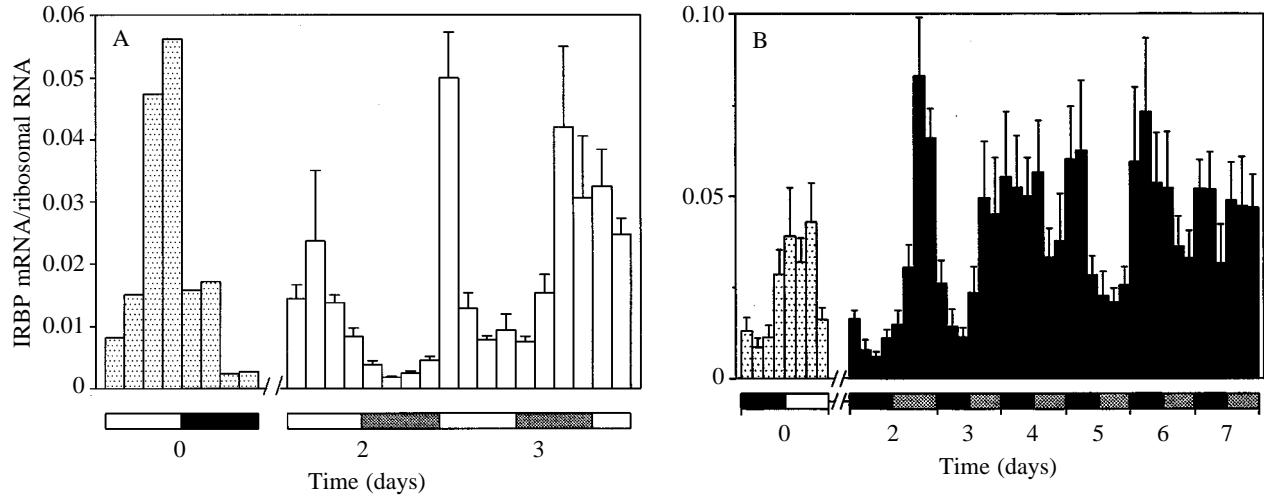
Fig. 10. Expression of the IRBP mRNA during constant conditions. Animals were cycled under 12 h:12 h light:dark (LD) for 2 weeks. On the last day of cyclic light, fish were killed every 3 h. Remaining fish were then exposed to constant conditions (constant light, LL; constant dark, DD). After 1 day of LL or DD, fish were killed every 3 or 4 h for the number of days shown. Error bars are standard errors of the mean. (A) Constant light. The stippled bars represent the mean value from fish during LD ( N=2 ). The white bars represent the mean value from fish during LL ( N=6 ). Horizontal bar under graph: open bar, light; filled bar, darkness; shaded bar, subjective night. (B) Constant dark. Stippled bars represent the mean value from fish during LD ( N=4 ). The black bars represent the mean value from fish during DD ( N=4 ). Horizontal bar under graph: open bar, light; filled bar, darkness; shaded bar, subjective day.
