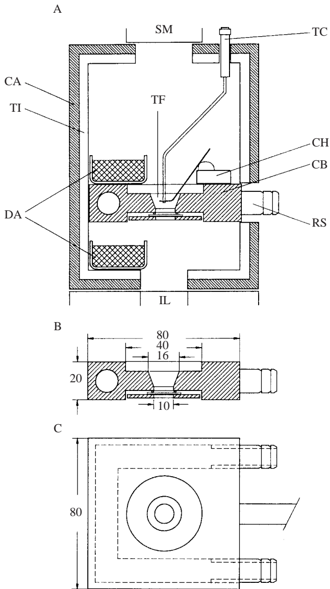
Fig. 3. Nanolitre osmometer. (A) Vertical section plan of the osmometer. (B) Cooling block, vertical section (plastic fixing rod not shown). (C) Cooling block from above. RS, refrigerant supply; IL, illumination; CA, cabinet; CB, cooling block; CH, capillary holder with a capillary cemented in place; SM, stereomicroscope; TC, thermocouple; TF, temperature-regulated fluid (90% ethanol); TI, thermoisolating layer; DA, drying agent (phosphorus pentoxide). In B and C, dimensions are given in mm.
