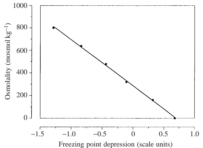
Fig. 4. Example of a calibration curve for the nanoliter osmometer shown in Fig. 3. Distilled water or solutions of NaCl of varying osmolality were used, and their freezing points determined.
