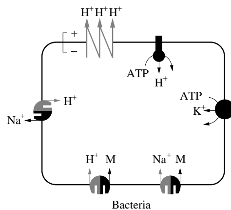
Fig. 1. In bacteria, the electron transport chain generates proton electrochemical gradients that drive both primary and secondary transporters that are located in plasma membranes. M, metabolite; Kdp, K^+ dependent.
