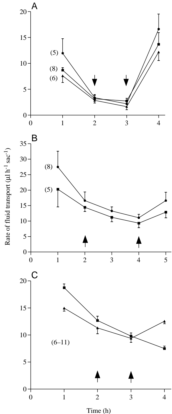
Fig. 6. Effect of Locusta migratoria diuretic hormone ( Locusta -DH) (filled squares; 10 \mu\text{mol l}^{-1} ) and locustakinin (Lom-K) (filled triangles; 10 \mu\text{mol l}^{-1} ) on the net rate of fluid transport measured hourly across everted ileal (A) and rectal (B,C) sacs of Schistocerca gregaria . After a control period (no treatment), neuropeptides were added (first arrow) for 1 or 2 h. Control preparations (filled circles) were not exposed to neuropeptides during this time. Finally, corpus cardiacum homogenate (1 gland-equivalent) was added in the last hour (second arrow) to test the responsiveness of all hindgut preparations. Bars show the means and vertical lines \pm 1 S.E.M. for the number of determinations shown in parentheses.
