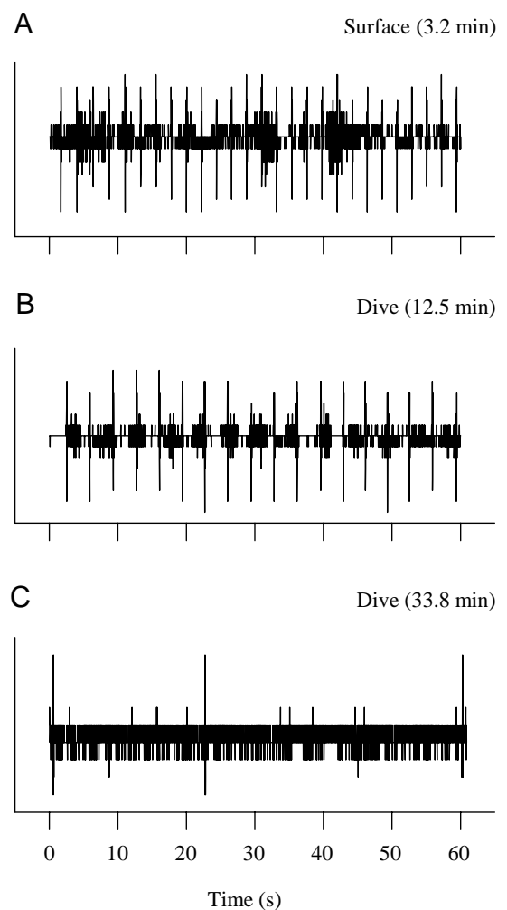
Fig. 5. Electrocardiogram (ECG) traces recorded from turtle 8866 during a surface interval of 3.2 min (A), a dive of 12.5 min (B) and a long-duration dive of 34 min (C). Mean heart rate during the 34 min dive was 3.6 beats min -1 , and heart beats occurred arrhythmically.
