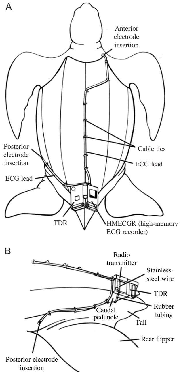
Fig. 1. Illustrations of data logger attachment to a leatherback sea turtle. (A) Dorsal view showing the placement of the data logger on the caudal peduncle and the electrode leads along the lateral ridges. (B) Left lateral view showing the data logger on the caudal peduncle and the posterior electrode insertion point. TDR, time/depth recorder.
