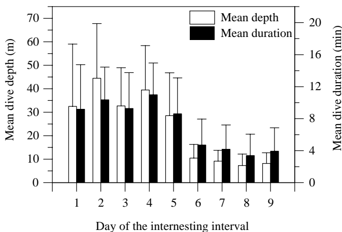
Fig. 3. Daily mean dive depth and mean dive duration over the interesting interval for turtle 7610. Dives are significantly deeper and longer during the first 5 days of the interesting interval compared with the last 4 days of the interval (Mann–Whitney rank test, P<0.05 ). Values are means + S.D.
