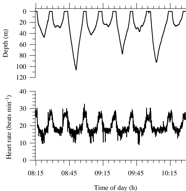
Fig. 6. A 2 h extract from a dive trace and the corresponding heart rate trace for turtle 7610. Although the depth and duration of the dives varied considerably, the heart rate response during diving was consistent. Heart rate dropped to a mean value of 16–17 beats \text{min}^{-1} during all dives illustrated.
