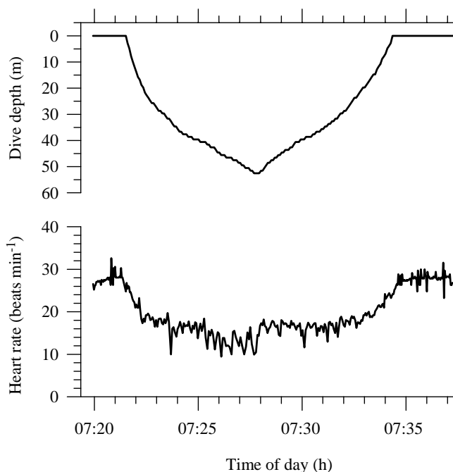
Fig. 4. Dive trace and corresponding heart rate trace for a single dive made by turtle 7610. Heart rate dropped as soon as the turtle submerged and continued to decline during descent. By mid-dive, the heart rate had stabilized between 15 and 17 beats min -1 . An increase in heart rate occurred during the ascent.
