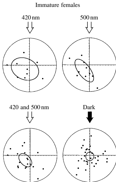
Fig. 5. Average orientations of immature females treated with 420 and 500 nm stimuli at an optical density of 0 (for corresponding intensity, see Table 1) in series 2 experiments. Mean vectors are pooled in the lower left figure. Each mean vector is calculated from orientations measured during the last 8 min of 10 min treatment periods. For corresponding statistical analyses, see Table 3.
