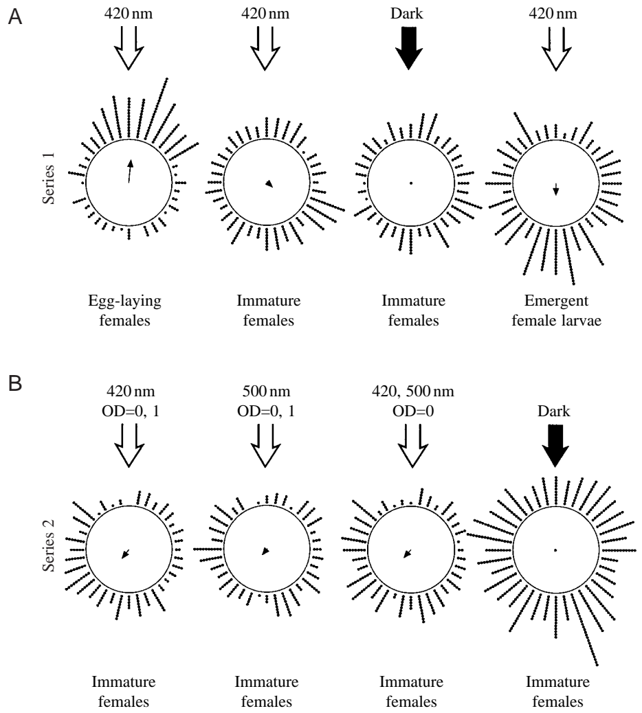
Fig. 2. Distribution of neck orientations measured at 30s intervals relative to the direction of monochromatic light. Mean vectors plotted within each circular histogram point in the mean direction, and their lengths indicate the concentration of observations in that direction (radius of circle 1.0). For corresponding statistical analyses, see Table 1. (A) Series 1 results. All treatments illustrated are at 420 nm and optical density (OD)=0. (B) Series 2 results. Different wavelength and intensity treatments are pooled in various combinations. See footnote of Table 1 for intensities corresponding to optical densities of 1 and 0 at each wavelength.
