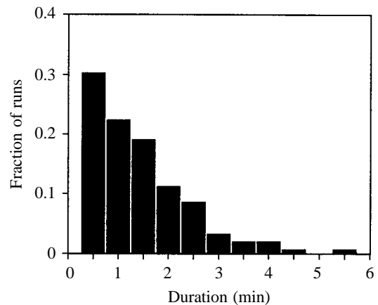
Fig. 3. Frequency distribution of run durations in the dark. The duration of runs of successive neck orientations falling within a 100^\circ range was determined for 10 immature worms over 8 min measurement periods. 152 runs were identified among 429 neck orientations measured.
