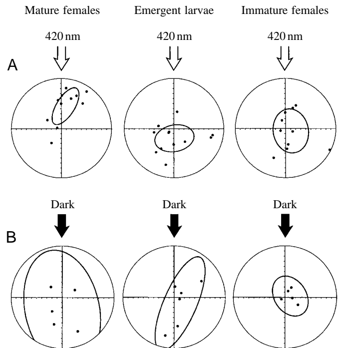
Fig. 4. Average orientations of females at the three stages of development tested in series 1 experiments. (A) Stimuli at 420 nm and optical density (OD)=0 (for corresponding intensity, see Table 1); (B) dark controls. Filled circles mark the tips of mean vectors with roots at the axis origin. Each mean vector is calculated from neck orientations measured during the last 26 min of 30 min treatment periods. The maximum possible vector length is 1.0, the radius of the circle. The Hotelling's confidence ellipse encloses the 95% probable location of the population mean vector tip. For corresponding statistical analyses, see Table 2.
