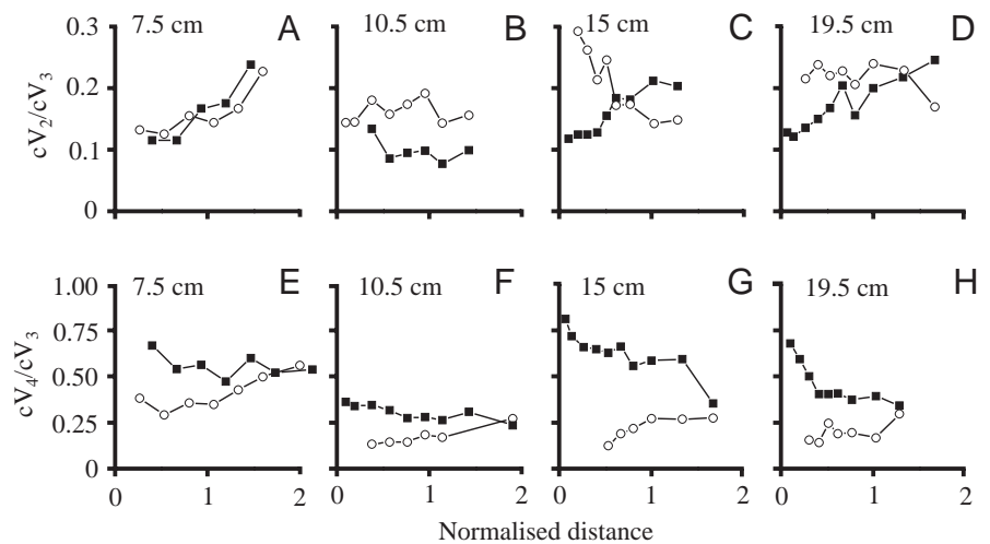
Fig. 9. The time waveform of the conspecific-generated local electric-organ-discharge-associated field (cLEOD) depends on the distance, size and orientation of the emitter fish. Data obtained from the same fish as in Fig. 8 (the emitting fish ranged from 7.5 to 19.5 cm in length, the receiving fish was 12 cm long). (A–D) The ratio cV_2/cV_3 as a function of distance between fish (normalised to the length of the emitting fish). (E–H) The ratio cV_4/cV_3 as a function of distance between fish (normalised to the length of the emitting fish). (○) Fish in parallel orientation; (■) fish in anti-parallel orientation. For an explanation of the nomenclature, see Fig. 1.
