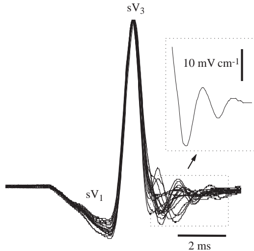
Fig. 3. Waveform coherence of the self-generated local electric-organ-discharge-associated field (sLEOD) at the electroreceptive fovea. For an explanation of the nomenclature, see Fig. 1. Normalised sLEOD time waveforms (average of eight sweeps) were obtained from 17 different positions located at the intersection of equally spaced parasagittal and transverse lines on the left hemifoveal region of a single fish. Note that the late oscillations due to the activity of peripheral elements of the electrosensory system vary from site to site but at each site are phase-locked to the sLEOD (a single trace, average of eight sweeps, is shown in detail in the inset).
