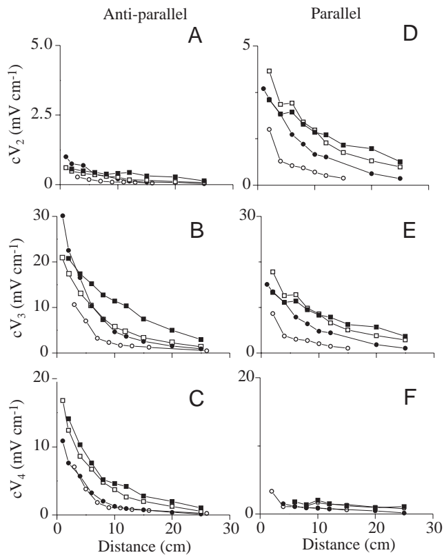
Fig. 8. Peak amplitudes of different time waveform components of the conspecific-generated local electric-organ-discharge-associated field (cLEOD) plotted as a function of distance between fish positioned anti-parallel and parallel. Emitter fish lengths: 7.5 cm (○), 11 cm (●), 15 cm (□) and 19.5 cm (■). Receiving fish length, 12 cm. (A) cV_2 , anti-parallel fish; (B) cV_3 , anti-parallel fish; (C) cV_4 , anti-parallel fish; (D) cV_2 , parallel fish; (E) cV_3 , parallel fish; (F) cV_4 , parallel fish. Note the different effects of anti-parallel and parallel orientations on cV_2 and cV_4 . For an explanation of the nomenclature, see Fig. 1.
