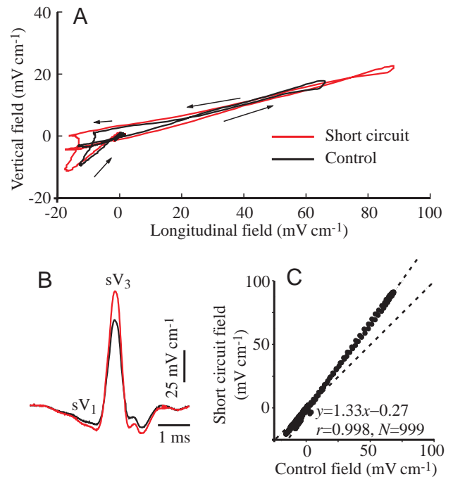
Fig. 4. Modulation of the self-generated local electric-organ-discharge-associated field (sLEOD) by a short circuit. A short circuit between two electrodes 0.5 cm and 3 cm in front of the skin caused changes in the nearby local field. The control condition is represented in black, and the short-circuit condition in red. (A) Local field vector loops of the sLEOD recorded at the midline of the jaw (foveal region) before and during the short circuit (average of eight sweeps). (B) Time waveforms of the sLEOD shown in A (average of eight sweeps). Simultaneous recordings of the head-to-tail electric-organ-discharge-associated field were not affected by the short circuit and were used as the time reference to align the recordings. (C) Short-circuit time waveform plotted against control time waveform. The slope of the line (1.33 in this case) is a measure of the amount of modulation ( r=0.998 , P<0.001 ). The reference broken line at 45^\circ corresponds to the no-change situation.
