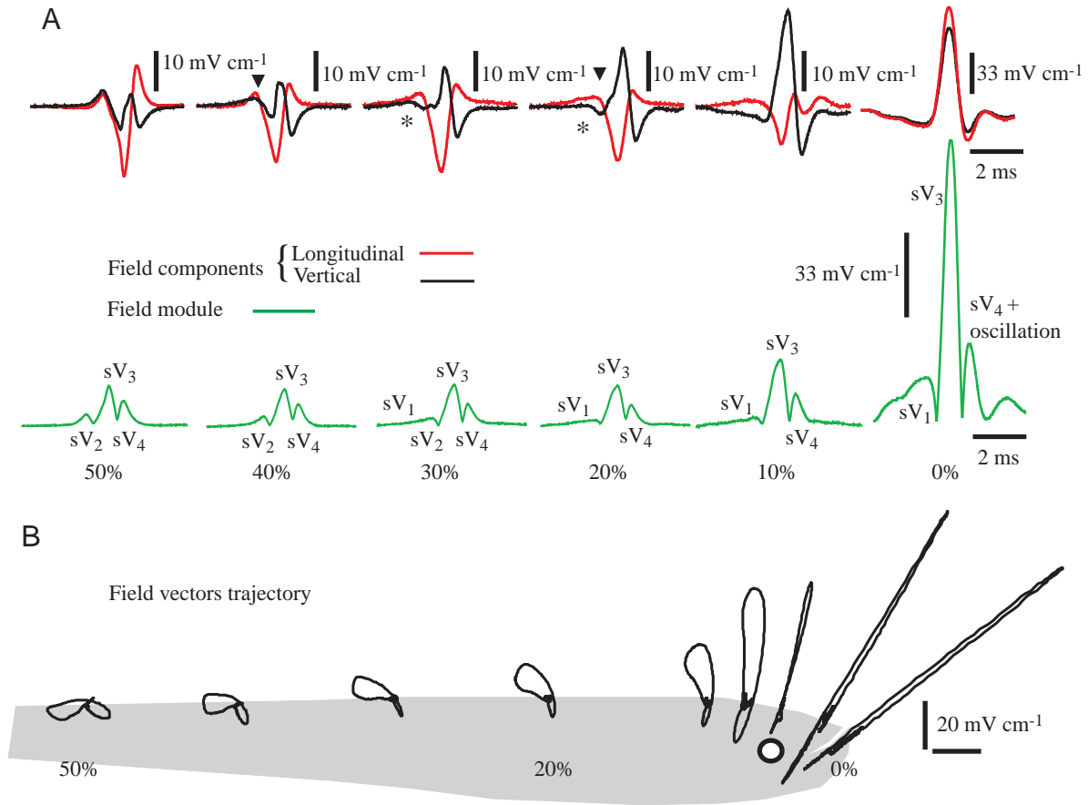
Fig. 2. General view of the spatio-temporal pattern of the self-generated local electric-organ-discharge-associated field (sLEOD). For an explanation of the nomenclature, see Fig. 1. (A) Recordings of vector components along the longitudinal (red traces) and vertical (black traces) axes and the local field modulus (green traces) obtained at six sites along the fish's midline (average of eight sweeps in each case). Distances from the jaw are expressed as a percentage of fish length. (B) Vector trajectories. Note that, in the head region, the local field components are similar (coherent) and therefore vector angles are time-independent. In the trunk region, the sLEOD components are different, so the field vectors describe a loop. For an explanation of asterisks and arrowheads, see text.
