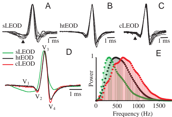
Fig. 10. Differences between the foveal self-generated local electric-organ-discharge-associated field (sLEOD), the foveal conspecific-generated local electric-organ-discharge-associated field (cLEOD) and the head-to-tail electric-organ-discharge-associated field (htEOD) time waveforms. Each trace is the average of eight sweeps. (A) Traces of the normalised sLEOD generated by 10 different fish (ranging in length from 7 to 24 cm). (B) Traces of the normalised htEOD obtained from the same 10 fish as in A. (C) Traces of the normalised cLEOD generated by 10 other emitting fish (emitting fish ranging in length from 7 to 24 cm, receiving fish 12 cm long). Note that superimposed traces shown in A, B and C were aligned and normalised to the peak of V_3 . The relative amplitude of V_1 mentioned in the text was measured 1.3 ms before the peak of V_3 (arrowheads in A and C). (D) Normalised time waveforms for the sLEOD (green), htEOD (black) and cLEOD (red) generated by a 22 cm emitting fish; the cLEOD was recorded at the fovea of a parallel 14 cm long fish, 10 cm away. (E) Normalised power spectral density histograms corresponding to the waveforms in D (same colour coding).
