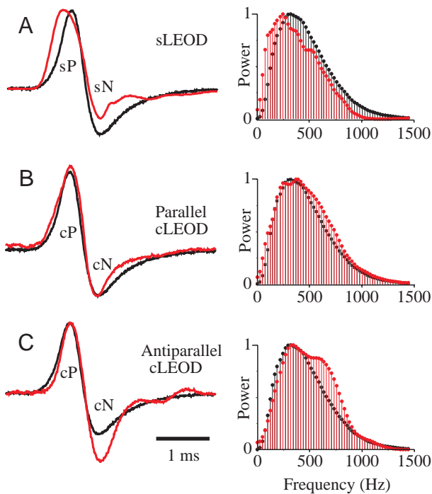
Fig. 13. The self-generated local electric-organ-discharge-associated field (sLEOD), the conspecific-generated local electric-organ-discharge-associated field (cLEOD) and the head-to-tail electric-organ-discharge-associated field (htEOD) time waveforms and power spectral densities of Brachyhypopomus pinnicaudatus . Each trace is the average of eight sweeps. Time waveforms are presented on the left and power spectral density histograms on the right. (A) The foveal sLEOD (red) and htEOD (black) from a 17 cm long male. (B) The cLEOD (red) generated by a 17 cm long male emitting fish at the fovea of a 20 cm long male receiving fish placed 7 cm away from and parallel to the emitting fish. The htEOD of the emitting fish is shown for comparison (black). (C) Same two fish as in B, but in the anti-parallel orientation, with the fish separated by 7 cm. The cLEOD is shown in red and the htEOD at the emitting fish in black (cP, the initial positive component; cN, the later negative component).
