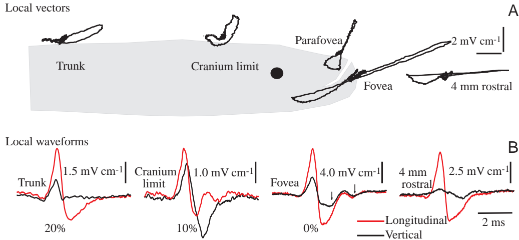
Fig. 5. General view of the spatio-temporal pattern of the conspecific-generated local electric-organ-discharge-associated field (cLEOD) at the midline of a receiving fish, when the emitter fish was placed antiparallel and 7 cm away. Vector trajectories (single sweeps, A) and LEOD longitudinal (red) and vertical (black) components (single sweeps, B) obtained at four sites adjacent to the skin are compared with the components of the local field obtained when the electrode was placed 4 mm away from the skin. Recording sites are as marked; distances from the fovea are measured as a percentage of fish length. Arrows mark the oscillations generated by the electroreceptor responses to the cLEOD.
