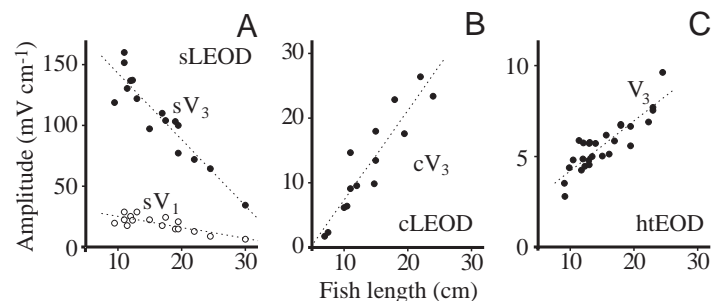
Fig. 11. Amplitude of the foveal self-generated local electric-organ-discharge-associated field (sLEOD) (A), of the conspecific-generated local electric-organ-discharge-associated field (cLEOD) (B) and of the head-to-tail electric-organ-discharge-associated field (htEOD) (C) as functions of the length of the emitting fish. In the case of the sLEOD, the peak of the two principal components is plotted ( sV_3 ●, sV_1 ○). Note that sV_1 and sV_3 of the sLEOD decrease with fish length, whereas cV_3 of the cLEOD and V_3 of the htEOD increase with fish length. For an explanation of the nomenclature, see Fig. 1. Suffixes 's' and 'c' indicate self- and conspecific-generated fields, respectively.
