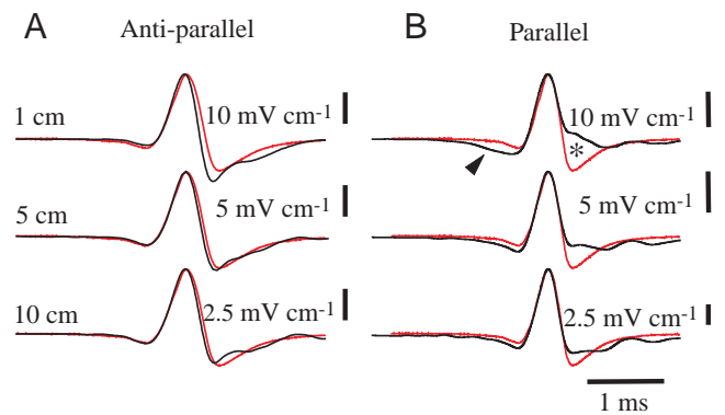
Fig. 7. Normalised conspecific-generated local electric-organ-discharge-associated field (cLEOD) (black) in anti-parallel (A) and parallel (B) oriented fish, with the head-to-tail electric-organ-discharge-associated field of the emitter fish (red) for comparison. Each trace is the average of eight sweeps. Time waveforms of cLEOD amplitude at the fovea of a 12 cm long receiving fish generated by a 15 cm long emitter fish at three different distances from the receiving fish (1 cm, 5 cm and 10 cm). Only when the fish were parallel and very close to each other was cV_1 obvious (arrowhead) and cV_4 practically absent (asterisk); for an explanation of the nomenclature see Fig. 1.
