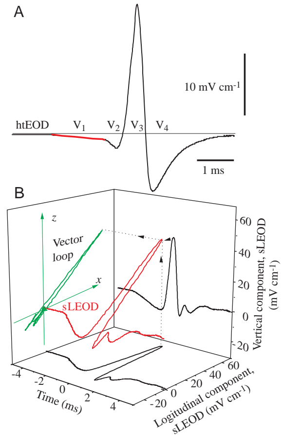
Fig. 1. (A) The head-to-tail electric-organ-discharge-associated field (htEOD) recorded between an electrode close to the head and another close to the tip of the tail (average of eight sweeps) of Gymnotus carapo . The wave components (terminology according to Trujillo-Cenóz et al., 1984) have been labelled [ V_1 (red), V_2 , V_3 and V_4 ]. (B) A plot showing the relationships between some of the different displays used in this paper. Local electric-organ-discharge-associated field (LEOD) components were recorded at selected points on the skin, and the LEOD waveform was calculated as a function of time (see Materials and methods). In this example, the data were obtained with the electrode placed at the midline, so the lateral local field component is virtually absent and is excluded from the representation for the sake of clarity. The third dimension has been used to represent time; ordinates are along the corresponding spatial directions. The black trace in the vertical plane corresponds to the vertical self-generated LEOD (sLEOD) component plotted as a function of time (average of eight sweeps). The black trace in the horizontal plane corresponds to the longitudinal sLEOD component as a function of time (average of eight sweeps). Dotted lines indicate how pairs of data obtained simultaneously at the peak of V_3 determine the amplitude and orientation of the corresponding local field vector at this time (peak points on the red and green traces). The local field obtained using this procedure is plotted over time in red (the time waveform, labelled sLEOD) and as a vector loop in green (projected onto the sagittal plane defined by the x and z axes).
