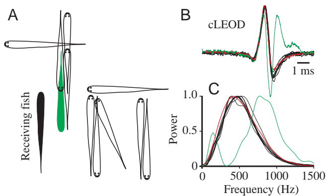
Fig. 6. The normalised conspecific-generated local electric-organ-discharge-associated field (cLEOD) generated by an emitter fish 14 cm long (black outline fish) at the fovea of a receiving fish 12 cm long (black solid fish); an average of eight sweeps in each case. Eleven different orientations shown diagrammatically in A are compared in this example. Foveal cLEODs represented by their normalised time waveforms (B) and their normalised power spectral density histograms (C). Note the similarity of waveforms and power spectral densities between the cLEOD (black lines) and the head-to-tail electric-organ-discharge-associated field (red lines). Interestingly, when the emitter fish was positioned as represented by the 'green' fish in A, the waveform (green line and spectrum plot) was very different from waveforms obtained at other orientations.
