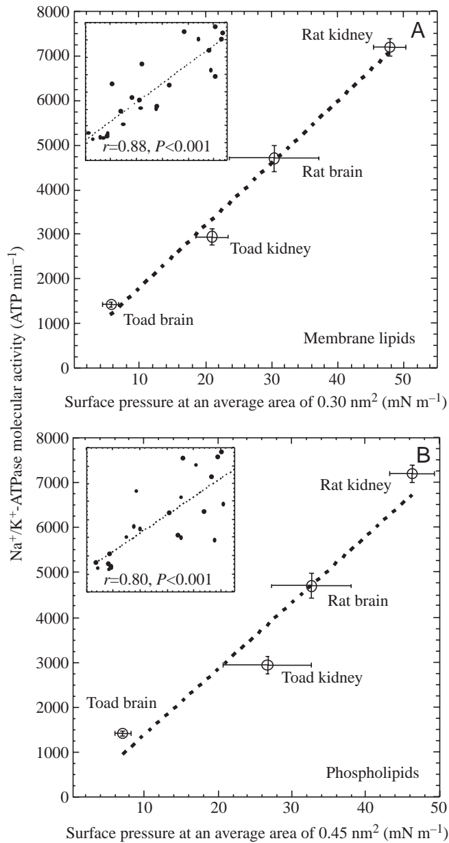
Fig. 3. The relationship between the molecular activity of the sodium pump ( \text{Na}^+/\text{K}^+ -ATPase) and the surface pressure of (A) membrane lipids and (B) phospholipids from kidney and brain microsomes of rats ( Rattus norvegicus ) and cane toads ( Bufo marinus ). Surface pressures were calculated at an average molecular area (per lipid molecule) of 0.30 \text{ nm}^2 and 0.45 \text{ nm}^2 , respectively, for membrane lipids and phospholipids. Each symbol represents the mean \pm S.E.M. of six determinations. Each inset graph shows the relationship for the 24 individual data points.
