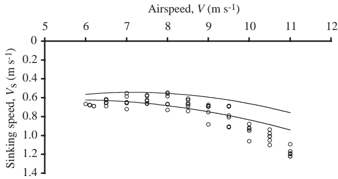
Fig. 13. Maximum performance during forward gliding flight for a jackdaw flying in a windtunnel. The upper curve is the maximum performance curve calculated according Pennycuick (Pennycuick, 1989) and using equation 12 to calculate the wingspan ratio. The lower curve is calculated according to the same theory, but instead using equations 17, 19 and 21 to calculate wingspan and area at different speeds. Parameter values were k (induced drag factor)=1.1, C_{D,par} (parasite drag coefficient)=0.1 and C_{D,pro} (profile drag coefficient)=0.014.
