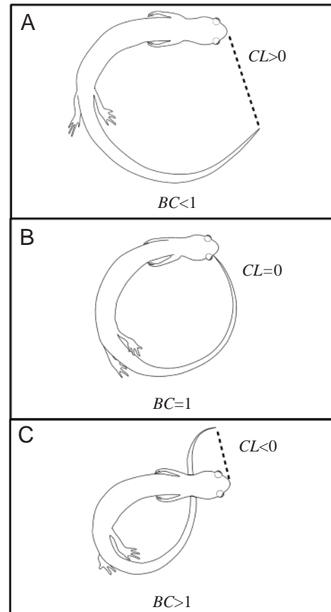
Fig. 1. Bending coefficient. Dorsal view of salamanders at maximum curvature demonstrating three escapes (A–C) with varying bending coefficients. Bending coefficient ( BC ) is defined as the ratio of head-to-tail chord length ( CL ; dashed line) to total length ( TL ) subtracted from 1: BC=1-(CL/TL) . To view video clips of escape responses, refer to the supplemental information section of the Journal of Experimental Biology website ( http://jeb.biologists.com ).
