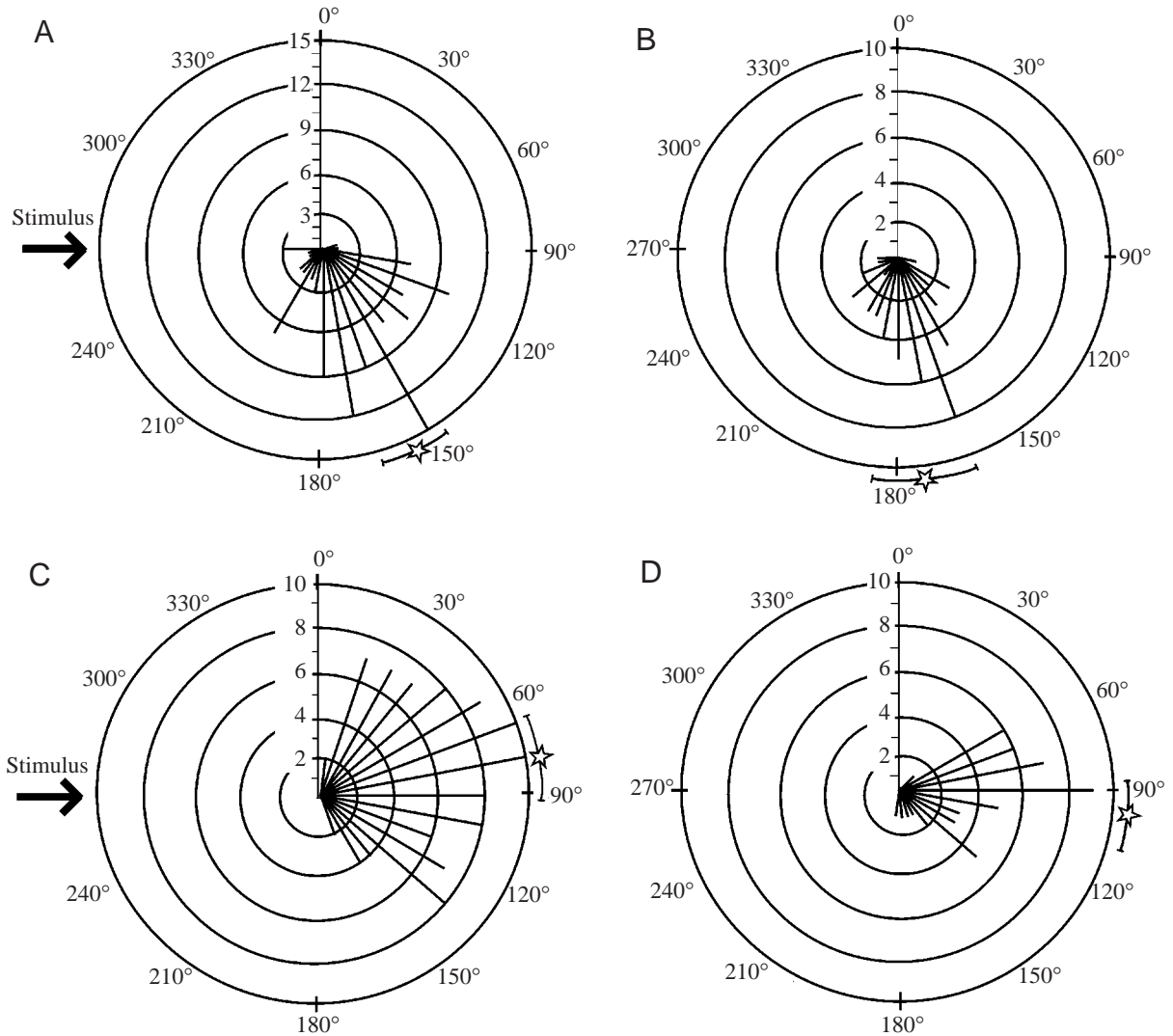
Fig. 6. Polar histograms showing the distribution of head angle at the end of stage 1 (stage 1 angle) (A,B) and stage 2 (final escape angle) (C,D) respectively for larvae (A,C) ( N=108 ) and adults (B,D) ( N=51 ). The number of escapes within 10^\circ intervals increases linearly. The data are standardized so that the salamander's head is initially aligned at 0^\circ , the stimulus is at 270^\circ and all escapes begin in the clockwise direction. For each polar plot, all escapes from a given life stage are pooled. Stars represent mean values for each life stage and error bars are 95% confidence intervals. The 95% confidence intervals for the mean final escape angle of both larvae (C) and adults (D) overlap with 90^\circ , indicating that neither is significantly different from 90^\circ .
