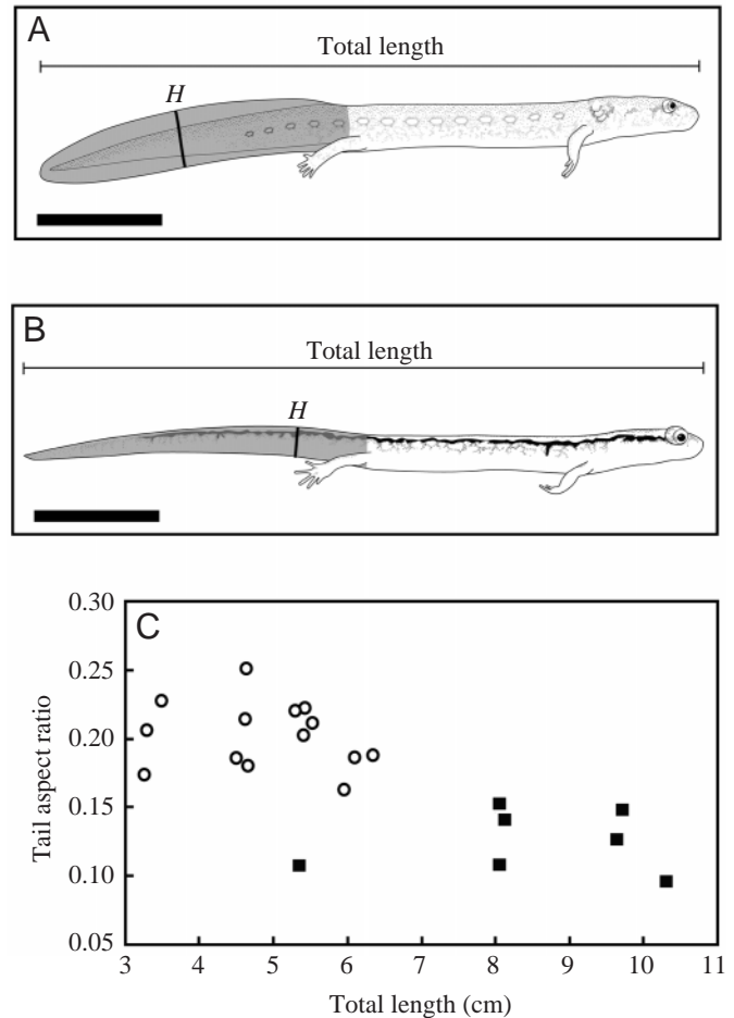
Fig. 2. Lateral view of larval (A) and adult (B) Eurycea bislineata . Tail aspect ratio ( \mathcal{A} ) is defined as the ratio of the square of maximum tail height ( H ) to lateral surface area ( LSA ) of the tail (shaded); \mathcal{A} = H^2/LSA . (C) Aspect ratio versus total length. Aspect ratio differs significantly ( P=0.0007 ) between larvae ( \circ ) and adults ( \blacksquare ) but is not significantly correlated with total length ( P=0.4593 ; one-factor ANCOVA). Scale bar, 1 cm.
