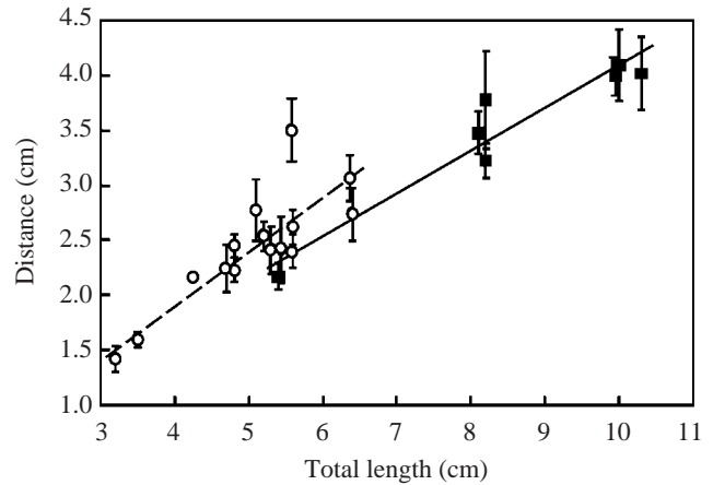
Fig. 5. Distance covered in stage 2 versus total length. Mean values calculated for each individual are plotted \pm S.E.M. ( N=7-11 escapes). Equations of linear regressions for stage 2 distance are y=0.482x+0.0097 ( r^2=0.69 , P=0.0002 ) for larvae (open circles and dashed line) and y=0.380x+0.274 ( r^2=0.91 , P=0.0008 ) for adults (filled squares and solid line). Distance travelled in stage 2 does not differ significantly between the two life stages ( P=0.196 ). Stage 2 distance is significantly positively correlated with total length.
