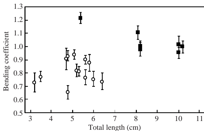
Fig. 3. Mean bending coefficient ( \pm S.E.M., N=7-11 escapes) for each individual plotted against total length. Bending coefficient differs significantly ( P=0.0007 ) between larvae (○) and adults (■) but is not significantly correlated with total length ( P=0.1767 ; one-factor ANCOVA).
