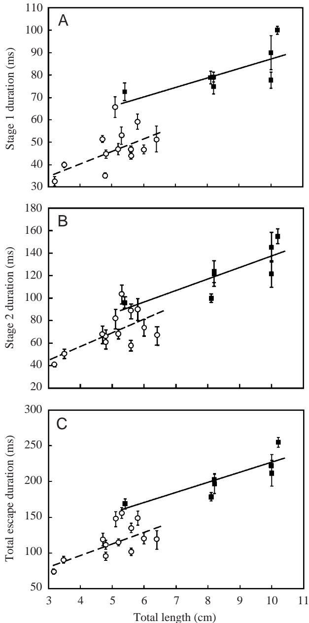
Fig. 4. Stage 1 duration (A), stage 2 duration (B) and total escape duration (C) versus total length. Mean values calculated for each individual are plotted \pm S.E.M. ( N=7-11 escapes). Equations of linear regressions for stage 1 duration are y=5.45x+19.8 ( r^2=0.32 , P=0.051 ) for larvae (open circles and dashed lines) and y=4.03x+47.2 ( r^2=0.50 , P=0.076 ) for adults (filled squares and solid lines). Equations of linear regressions for stage 2 duration are y=11.5x+12.1 ( r^2=0.38 , P=0.025 ) for larvae and y=10.3x+34.8 ( r^2=0.663 , P=0.026 ) for adults. Equations of linear regressions for total escape duration are y=16.9x+31.9 ( r^2=0.40 , P=0.02 ) for larvae and y=14.3x+82.1 ( r^2=0.72 , P=0.016 ) for adults. For results of one-factor ANCOVA, refer to Table 2.
