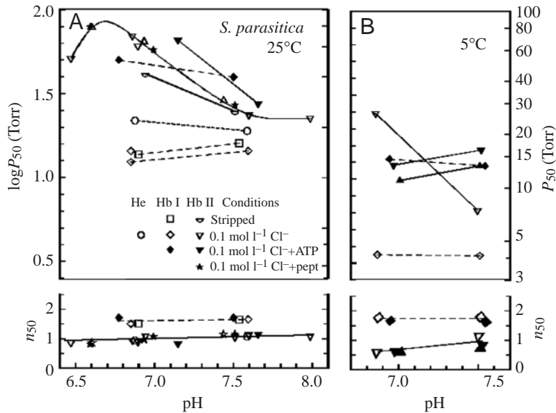
Fig. 3. P_{50} ( O_2 tension at half O_2 saturation) and n_{50} (Hill cooperativity coefficient at P_{50} ) values of Symenchelis parasitica hemolysate (He, dotted line), Hb I (dashed lines) and Hb II (continuous lines) and their pH dependence in the absence of effectors and in the presence of 0.1 \text{ mol l}^{-1} KCl, saturating ATP levels and peptide corresponding to the 10-mer amino-terminal segments of the cytoplasmic domain of Band 3 protein (cd-B3) from trout red cell membranes (peptide/Hb tetramer molar ratio=5) measured at 25^\circ\text{C} (A) and 5^\circ\text{C} (B). Other conditions are as described in the legend to Fig. 2. (7.50 Torr=1 kPa.)
