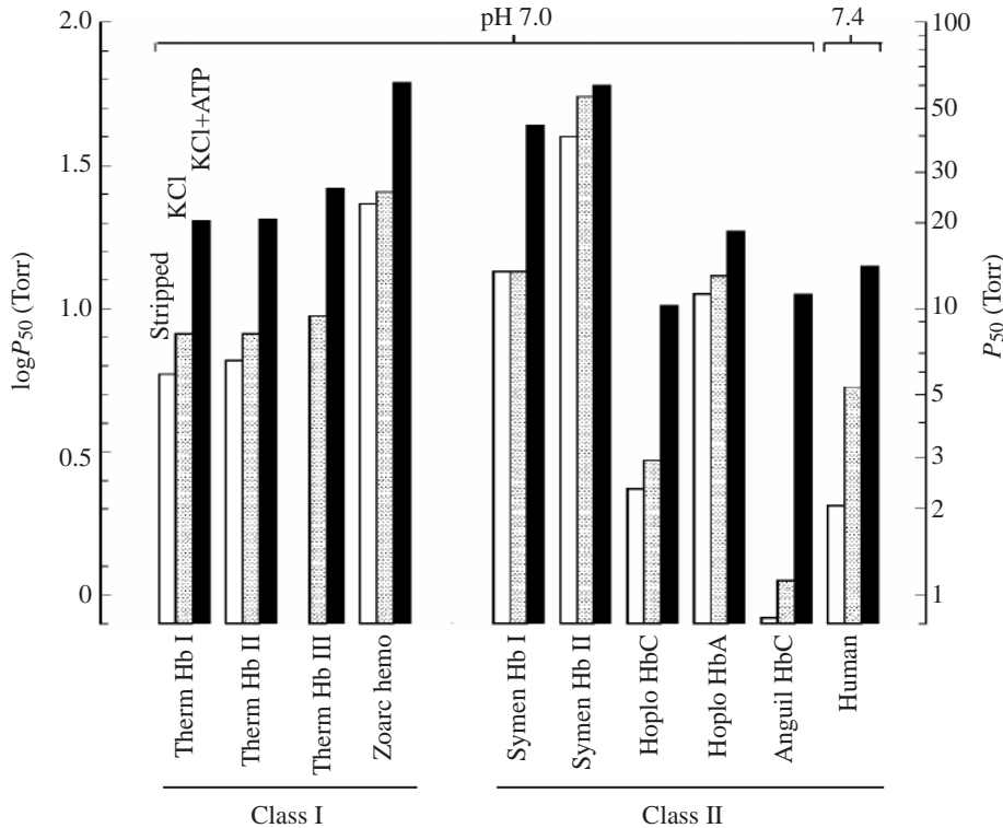
Fig. 8. P_{50} ( O_2 tension at half O_2 saturation) values of Thermarces cerberus (Therm) Hbs I and II and S. parasitica (Symen) Hbs I and II compared with those for Zoarc viviparus hemolysate (Zoarc), Hoplosternum littorale cathodic and anodic Hbs (Hoplo HbC and Hoplo HbA; Weber et al., 2000) and eel Anguilla anguilla cathodic HbC (Anguil HbC; Fago et al., 1995) at pH 7.0 and human Hb at pH 7.4 (Imai, 1982). Open columns, stripped Hbs; shaded columns, Hbs in the presence of 0.1 \text{ mol l}^{-1} KCl; solid columns, Hbs in the presence of 0.1 \text{ mol l}^{-1} KCl + saturating concentrations of ATP (fish Hbs) or 2,3-diphosphoglycerate (DPG; human Hb). Other conditions: 0.1 \text{ mol l}^{-1} Hepes buffer (fish Hbs) or 0.05 \text{ mol l}^{-1} Bis-Tris (Human Hb) and 25^\circ\text{C} ( 20^\circ\text{C} for Anguil HbC). ( 7.50 \text{ Torr}=1 \text{ kPa} .)
