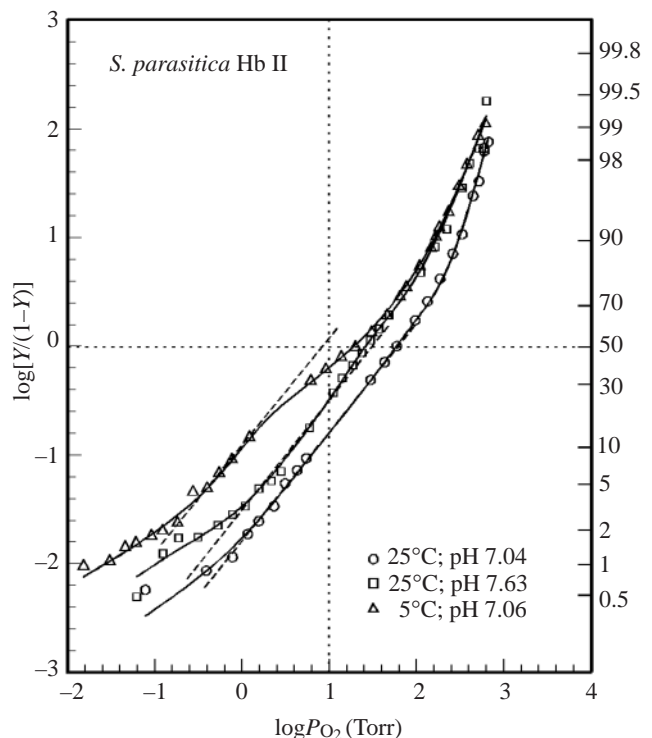
Fig. 4. Extended Hill plots (where Y is the fractional O_2 saturation) of S. parasitica Hb at pH 7.04–7.06 and either 5^\circ\text{C} (triangles) or 25^\circ\text{C} (circles) and at pH 7.63 and 25^\circ\text{C} (squares). The intercepts of the asymptotes to the lower parts of the curves (broken lines with slopes of unity) with the vertical axis at \log P_{O_2} indicate the K_T (the O_2 association constant of the low-affinity deoxy state of the molecules) values. Heme concentration, 0.80 \text{ mmol l}^{-1} . (7.50 Torr=1 kPa.)
