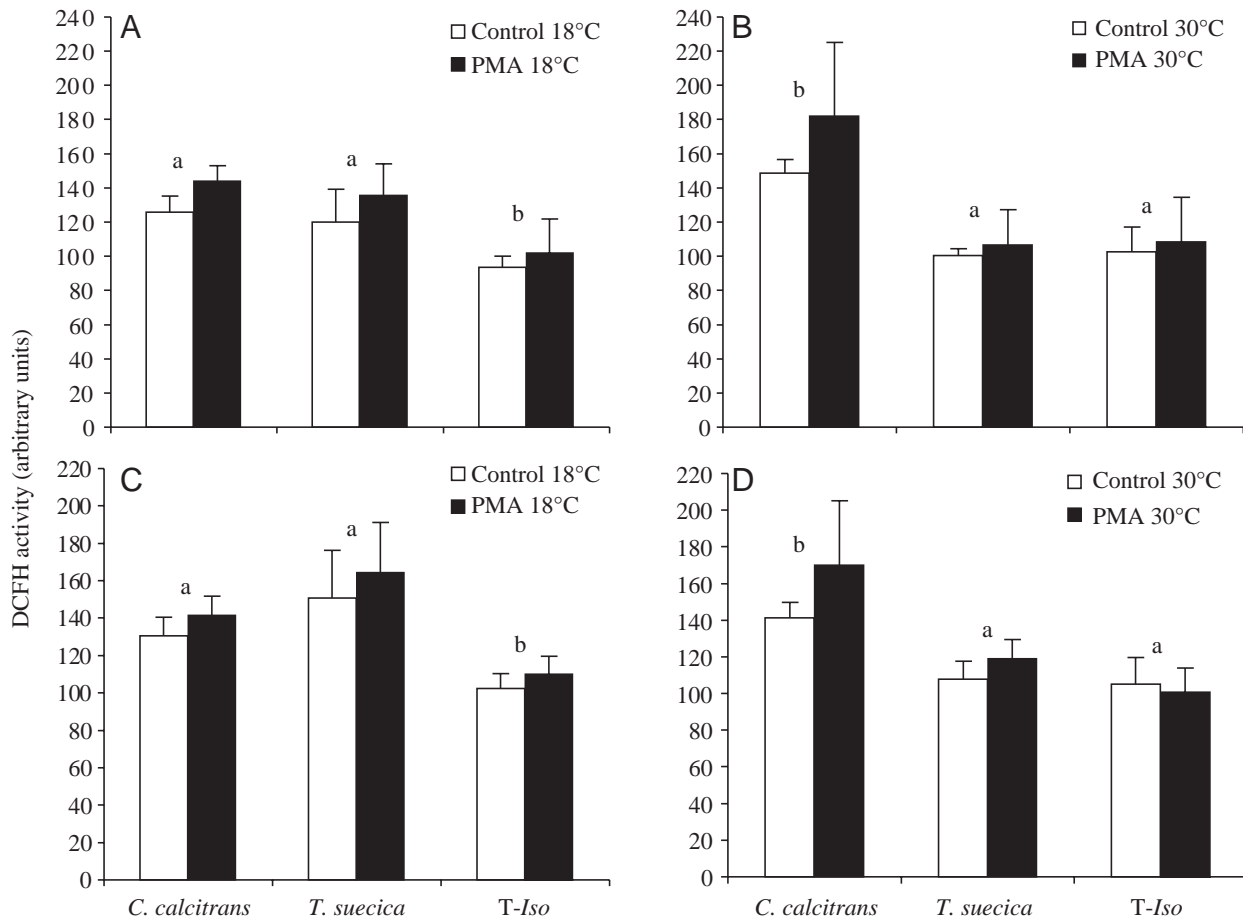
Fig. 4. 2'7'-dichlorofluorescein (DCFH) activity of oyster haemocyte sub-populations after 20 min of incubation with phorbol myristate acetate (PMA) and without PMA (control) at different temperatures: (A) granulocyte sub-population at 18°C; (B) granulocyte sub-population at 30°C; (C) hyalinocyte sub-population at 18°C; (D) hyalinocyte sub-population at 30°C. Different lower-case letters indicate significant difference between dietary treatments (mean \pm S.D.; N=3 ; ANOVA P<0.05 ). No effect of PMA stimulation was noted.
