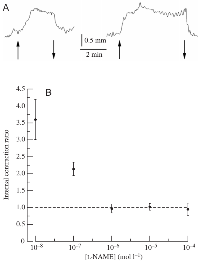
Fig. 6. The effect of L-NAME on internal contraction ratios. (A) Contractions of the same demibranch in response to 2 \times 10^{-5} mol l -1 5HT (applied at the upward arrows). The response to each dose of 5HT was terminated by flushing the organ bath (downward arrows). L-NAME ( 10^{-4} mol l -1 ) was applied for 15 min before the second contraction. The resulting internal contraction ratio was 0.92. (B) Various concentrations of L-NAME were applied to isolated demibranchs for 15 min between their first and second contractions in response to 2 \times 10^{-5} mol l -1 5HT. Values are means \pm 1 S.E.M., N=3 for all concentrations of L-NAME except 10^{-4} mol l -1 where N=4 .
