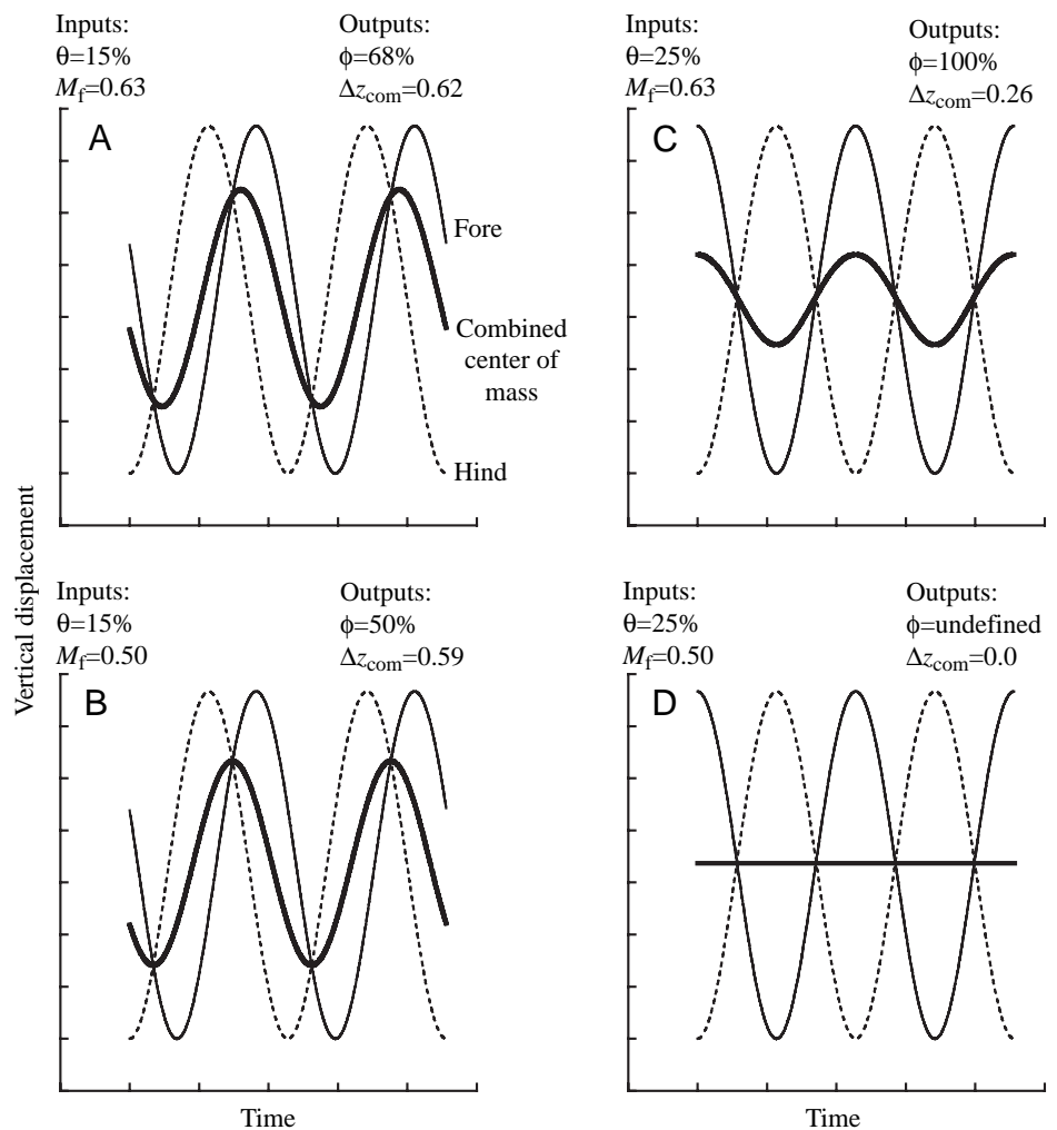
Fig. 5. Vertical displacement of the fore pendulum, hind pendulum and system center of mass versus time for specific examples from the two-pendulum model of quadrupedal walking. The model consists of two identical independent pendulums representing a quadruped's fore and hind quarters with a variable phase relationship ( \theta ) and mass distribution ( M_f ). \theta is the percentage of stride time that the fore pendulum displacement lags the hind pendulum displacement (analogous to the phase between a dog's ipsilateral fore and hind limbs), and M_f is the ratio of fore pendulum mass to the combined mass of both pendulums (equivalent to the fraction of body weight supported by the fore limbs). The time interval shown is equivalent to a complete dog stride. \Delta z_{com} is the magnitude of the center of mass vertical displacement relative to the pendulum displacement, and \phi is the time interval between the peak center of mass vertical displacement and the peak hind pendulum vertical displacement, expressed as a percentage of time between peak hind and fore pendulum displacements. A represents the pendulum phase and mass distribution combination actually used by the dogs, and D represents the phase and mass distribution shown in the hypothetical diagram of Fig. 1. B and C represent intermediate patterns.
