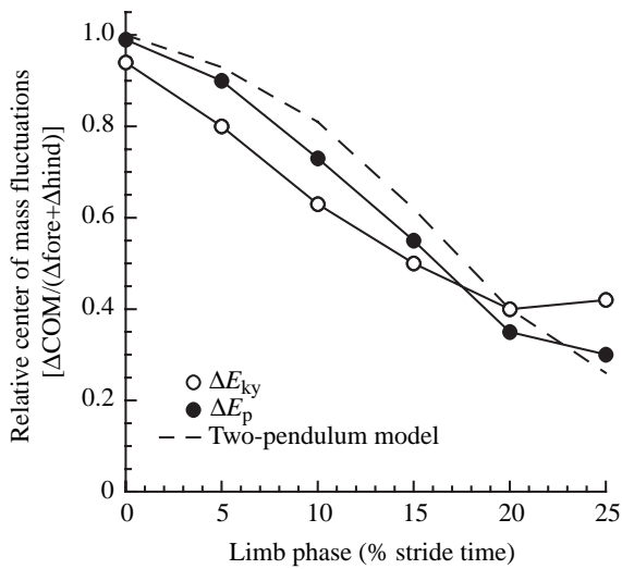
Fig. 10. Decreasing limb phase increased gravitational potential energy ( \Delta E_p ) and fore–aft kinetic energy ( \Delta E_{ky} ) fluctuations of the center of mass relative to those of the fore and hind quarters. As limb phase approached 0%, the vertical and fore–aft movements of the fore and hind quarters were more synchronous. These changes were similar to those predicted by the two-pendulum model. We assumed that (1) the fore and hind quarters were, respectively, 63% and 37% of the total mass (37.8 kg) and (2) limb phase did not affect the ground reaction force. Values were calculated using mean individual limb ground reaction force data for dogs walking at 0.8 \text{ m s}^{-1} (Fig. 8) and time-shifting the data to simulate a range of limb phases. The values for 15% limb phase correspond to the example in Fig. 9.
