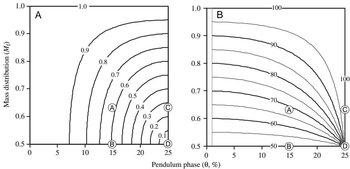
Fig. 6. Contour plots of the magnitude of the center of mass vertical displacement relative to the pendulum vertical displacement ( \Delta z_{com} ; A) and the phase relationship between the center of mass and the hind pendulum vertical displacement ( \phi ; B) for the two-pendulum model of walking. These data are plotted as a function of the relative mass of the fore pendulum, M_f , and the phase difference between the fore and hind pendulums, \theta . Both pendulums have the same amplitude in all cases. The circled letters correspond to the combinations of phase and mass distribution in Fig. 5A–D.
