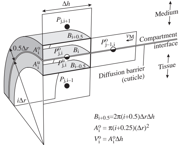
Fig. 4. Oxygen transfer across a compartment interface with additional diffusion barrier (cuticle). The grid point referenced by the indices i and j is located on an infinitesimal thin diffusion barrier separating the tissue from the medium compartment. This grid point is characterized by two variables, P_{j,i}^u and P_{j,i}^o , which represent the oxygen partial pressure at the inner and the outer side of the circular diffusion barrier, respectively. To calculate the temporal changes in P_{j,i}^u and P_{j,i}^o (see equations 4, 5), the following geometrical parameters are required: the cylindrical wall areas B_{i-0.5} , B_i and B_{i+0.5} , the areas of the hollow-cylindrical bases A_i^u and A_i^o , and the hollow-cylindrical volumes V_i^u and V_i^o . Three example equations for calculating these parameters are given. v_M , flow velocity in the medium compartment; P_{j,i-1} , P_{j,i+1} , P_{j-1,i}^o , oxygen partial pressures of the neighbouring grid points; \Delta h and \Delta r , distance between two grid points in axial and radial direction.
