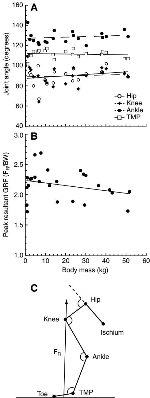
Fig. 2. (A) The mean joint angles at mid-stance versus body mass while running with a 0.40 duty factor (DF), for the hip (open circles), knee (closed diamonds), ankle (closed circles) and TMP joints (open squares). The equations for the least-squares regression lines ( \pm 95\% CI for the slope) are as follows: hip, y=87.3+0.13x ( \pm 0.24 , R^2=0.07 ); knee, y=88.9+0.04x ( \pm 0.30 , R^2=0.01 ); ankle, y=127.2+0.06x ( \pm 0.17 , R^2=0.03 ), and TMP, y=112.0-0.03x ( \pm 0.12 , R^2=0.01 ). (B) Peak resultant ground reaction forces ( F_R ) normalized by body weight when running with a 0.40DF; y=2.24-0.004x ( \pm 0.006 , R^2=0.08 ). (C) A scaled stick figure representation of the typical emu hindlimb posture at the time of peak bone strains when running with a 0.40DF. The joint angles (mean \pm s.d.) are as follows: hip, 86\pm 9^\circ ; knee, 97\pm 12^\circ ; ankle, 129\pm 7^\circ ; TMP, 120\pm 7^\circ . F_R is oriented 1.7^\circ from the vertical axis in the fore–aft plane, passing near the knee. Even though the TMP joint is inclined slightly relative to the toe ( 9^\circ ), the foot was flat on the ground at the time of peak bone strains.
