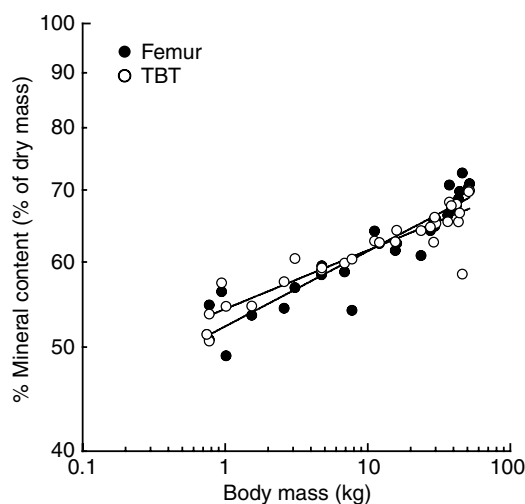
Fig. 11. Percent mineral content by mass versus body mass on logarithmic axes for the emu femur (closed circles) and TBT (open circles). Femur: y=52x^{0.070\pm 0.010} ( R^2=0.88 ); TBT: y=54x^{0.055\pm 0.009} ( R^2=0.83 ).
