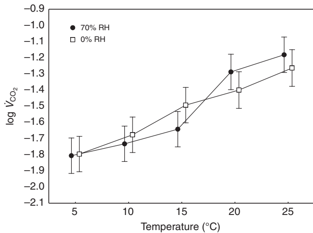
Fig. 4. Effects of temperature and humidity on standard metabolic rate ( \text{ml CO}_2 \text{ h}^{-1} ) of Peripatopsis capensis . Values are means \pm 95% confidence intervals.
