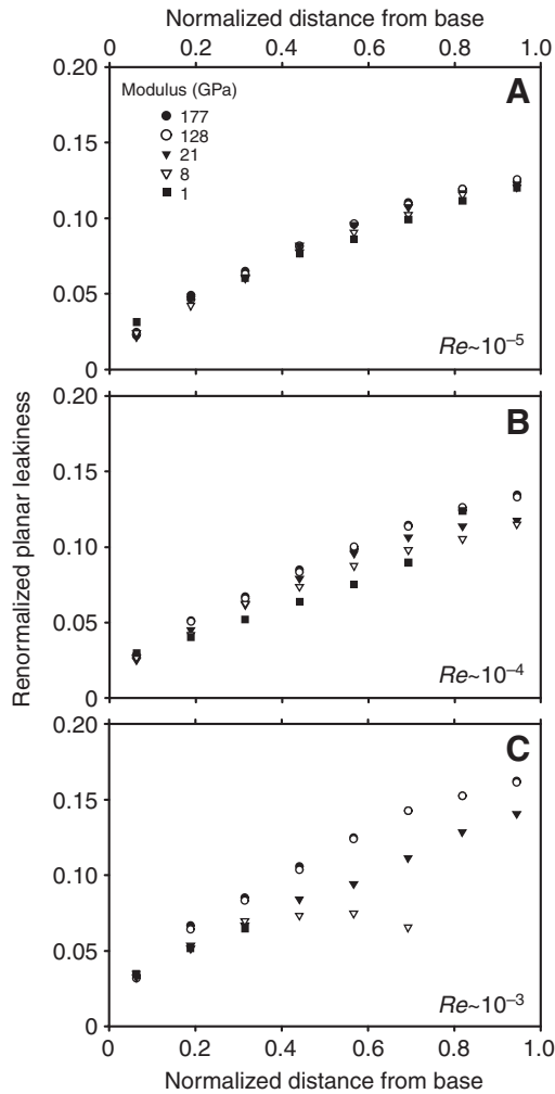
Fig. 7. Renormalized planar leakiness (i.e. calculated relative to instantaneous rather than idealized array width) versus distance from the base of filter arrays ( L/d=100 ) operating at approximate Re of (A) 10^{-5} , (B) 10^{-4} , and (C) 10^{-3} . Divergent trajectories evident in B and C illustrate changes in leakiness that were independent of variation in array width. Distances from the filter base were normalized by the height, L , of a stationary array.
