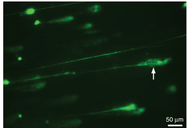
Fig. 4. Fluorescent tagging of mucins using a fluorescein-labeled lectin dye illustrates the formation of mucin strands from elongated mucin vesicles exposed to shear in a flow-through chamber. Arrow indicates an aggregation of ruptured mucin vesicles that have begun elongating to form strands.
