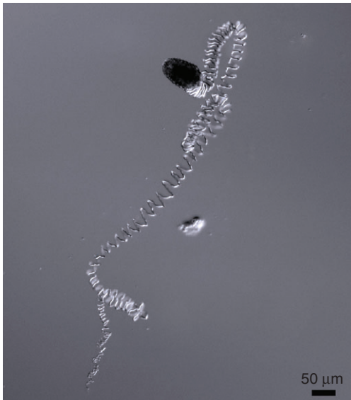
Fig. 1. Differential interference contrast (DIC) image of partially unraveled thread skein in seawater illustrating their coiled structure.
