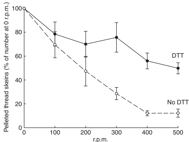
Fig. 3. Mean ( \pm s.e.m.) number of condensed thread skeins as a function of mixing rate expressed as the percentage of skeins at 0 r.p.m.. These data provide an inverse measure of the degree of thread skein unraveling in the whole slime. Solid line indicates data for trials in which mucins were disrupted with 10 \text{ mmol l}^{-1} dithiothreitol.
