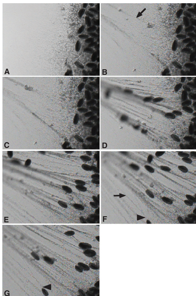
Fig. 5. Slime exudate exposed to flow created by a syringe pump. (A) Condensed exudate puddle prior to flow. Note the condensed thread skeins on the far right and the mucin vesicle boundary layer to the left. (B,C) Mucin strands and chains begin to form as flow is initiated. (D,E) Mucin strand attachment to thread skeins and movement of thread skeins. (F,G) Unraveling of thread skeins initiated. Arrowheads indicate an unraveling thread skein, arrows indicate aggregations of mucin strands.
