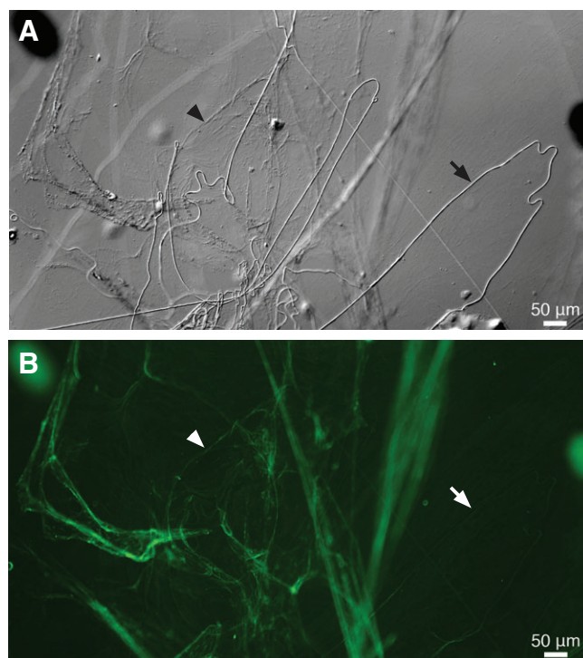
Fig. 6. Whole slime formed in seawater containing the fluorescent lectin dye (A) Differential interference contrast (DIC) image of whole slime network depicting unraveled threads and mucin strand network. Arrowhead indicates mucin strands connecting slime threads, and the arrow indicates a slime thread. (B) Same image viewed in fluorescence highlights the complexity of the mucin network.
