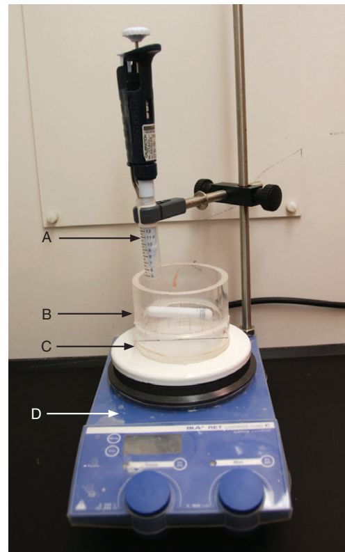
Fig. 2. Thread skein unraveling experimental apparatus. (A) Micropipette insertion guide, (B) experimental chamber with stir bar, (C) spacer and chamber alignment guide, (D) stir plate with feedback speed control.
