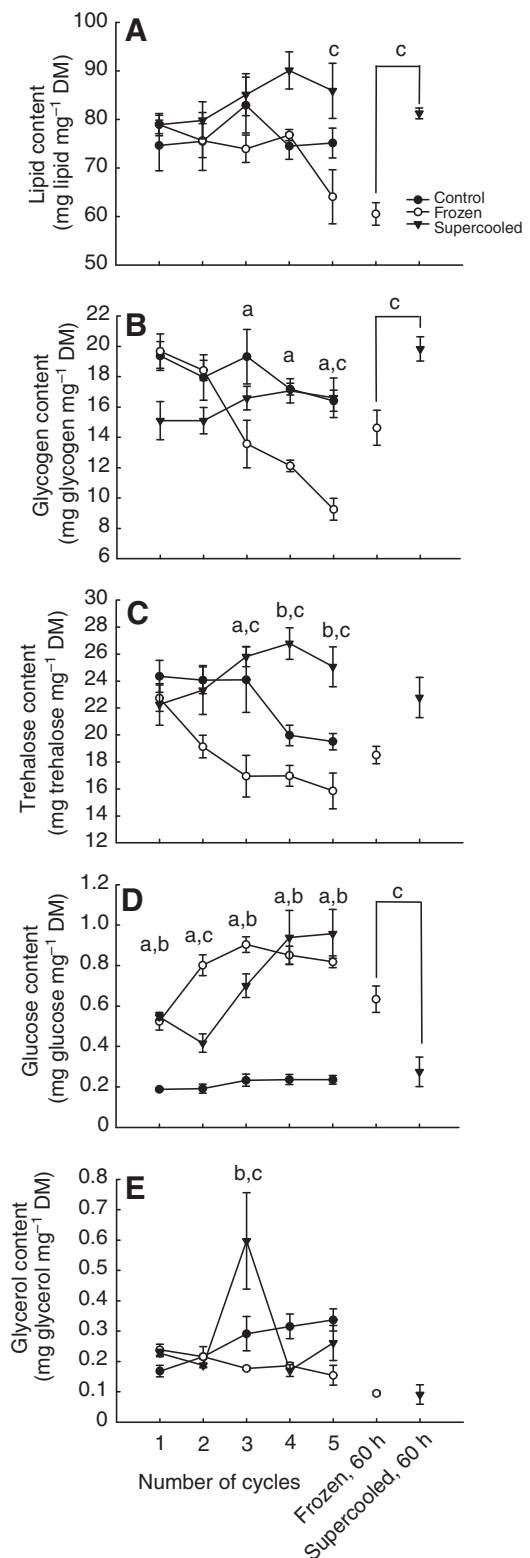
Fig. 2. (A) Lipid, (B) glycogen, (C) trehalose, (D) glucose and (E) glycerol content of B. antarctica larvae during RCE. Values are means \pm s.e.m. The metabolite content is based on the mean of five replicates, five larvae per replicate for the lipid analysis, 45 larvae per replicate for the other metabolites. At each time point, 'a' indicates a significant difference between control and frozen larvae, 'b' represents a significant difference between control and supercooled larvae, and 'c' represents a significant difference between frozen and supercooled larvae (ANOVA, Bonferroni, P < 0.05 ). DM, dry mass.
