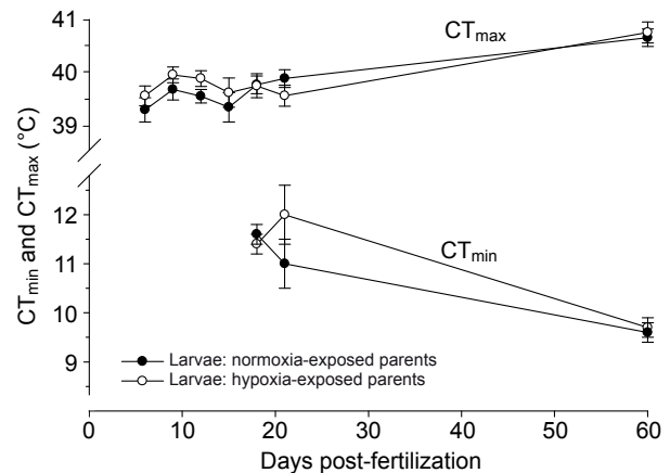
Fig. 7. Critical minimum thermal limit (CT min ) and maximum thermal limit (CT max ) of zebrafish larvae from parents reared in normoxia or hypoxia for 12 weeks. CT min and CT max were not significantly different between treatment groups (two-way ANOVA with Tukey's post hoc analyses, P > 0.05 ). N = 8–12 for each group at each time point. Mean values \pm 1 s.e.m. are presented.
