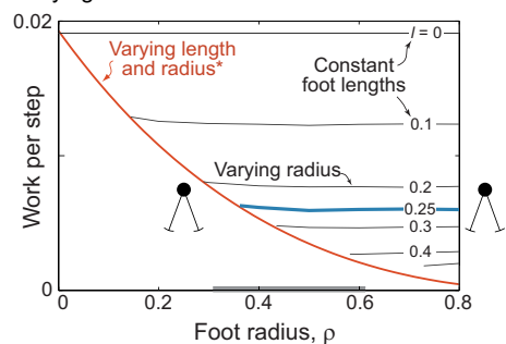
Fig. 2. Dynamic walking model predictions for step-to-step transition work as a function of foot radius and length. (A) Step-to-step transition work per step (vertical axis) depends on both arc radius and length, the latter having a much greater effect. (B) Work decreases nearly quadratically as a function of foot length, as demonstrated for various foot radii. (C) In contrast, work per step varies little with foot radius, as shown for various foot lengths. The approximate range of experimental conditions is denoted by the shaded area on the horizontal axes. Filled circles in A show the parameters studied experimentally (see Fig. 3). In B and C, the boundary of the parameter space for the current model shows results that agree closely with a previous model, in which length and radius varied together (Adamczyk et al., 2006).
