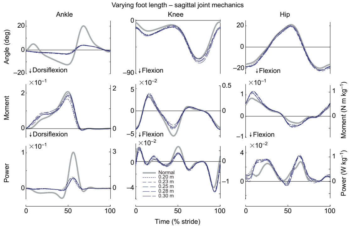
Fig. A1. Sagittal joint mechanics (angle, moment, power output) across variations in foot length. Curves are averaged across all eight subjects. Values are nondimensionalized on the left-hand axes; values on the right-hand axes units are normalized to body mass.
