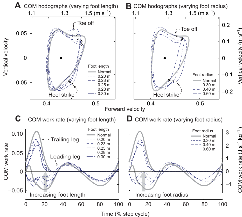
Fig. 5. (A,B) Vertical versus forward components of center of mass (COM) velocity data, termed COM hodographs, for arc feet of varying (A) length and (B) radius. (C,D) COM work rate versus step cycle for varying (C) foot length and (D) foot radius. Curves are shown for both legs (labeled as leading and trailing leg during step-to-step transition). All curves are averaged across subjects ( N=8 ).
