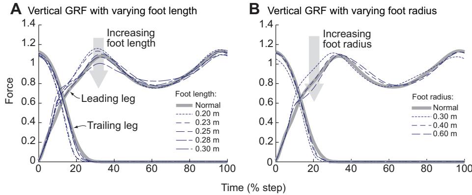
Fig. 4. Average ground reaction force data over a step cycle, for varying (A) foot length keeping radius fixed and (B) foot radius keeping length fixed. Curves are averaged across all ( N=8 ) subjects. A step was defined as starting at one heelstrike and ending at opposite heelstrike.
