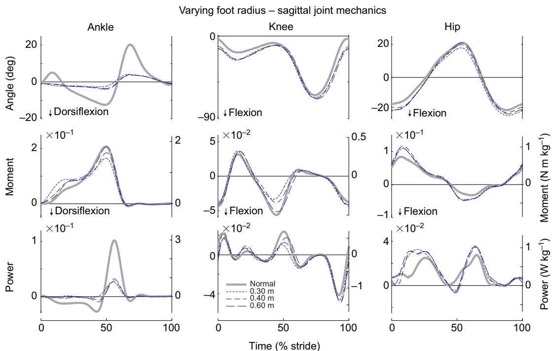
Fig. A2. Sagittal plane joint mechanics (angle, moment, power output) across variations in foot radius. Curves are averaged across all eight subjects. Note the trend toward increasing knee moment in late stance, which may reflect the altered timing of GRF center of pressure advancement due to changing foot radius. Values are nondimensionalized on the left-hand axes; values on the right-hand axes units are normalized to body mass.
