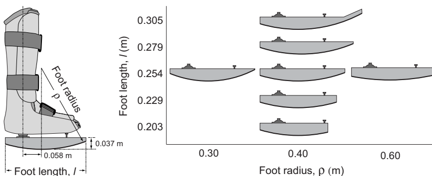
Fig. 3. Apparatus used to impose an arc-like shape to the foot bottom, while keeping the ankles fixed (see also Adamczyk et al., 2006). Arcs were constructed in five lengths and three radii of curvature.
