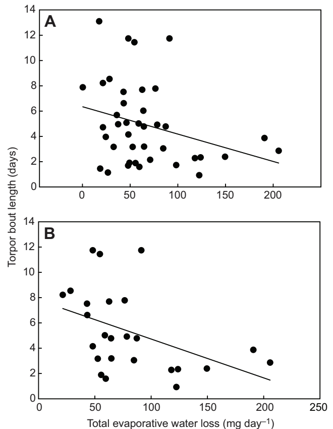
Fig. 1. Relationship between torpor bout length (TBL) and total evaporative water loss (TEWL) in Kuhl's pipistrelle measured while (A) torpid in either dry or humid air conditions (TBL=6.35–0.02 \times TEWL, R^2=0.09 , P=0.05 ) and (B) torpid in dry air ( T_a=5^\circ\text{C} : 0.41 \pm 0.30 g H 2 O m -3 , RH=6%; T_a=10^\circ\text{C} : 0.58 \pm 0.05 g H 2 O m -3 , RH=6%; TBL=1.99–0.006 \times TEWL, R^2=0.20 , P=0.02 ).
