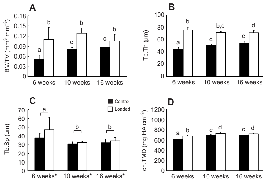
Fig. 3. Changes in cancellous tissue of the proximal tibial metaphyses with applied load for 6-, 10- and 16-week-old mice. (A) Bone volume fraction, BV/TV, (B) trabecular thickness, Tb.Th, (C) trabecular separation, Tb.Sp, and (D) cancellous tissue mineral density, cn.TMD. Values shown are means + 1 s.d. Data for the control and loaded tibiae are shown in black and white, respectively. The letters above the bars (or bracketed pairs of bars) indicate a statistically significant difference ( P < 0.05 ) between groups with different letters and no difference between groups with the same letters, by linear mixed model with repeated measures, followed by pairwise comparisons with Bonferroni correction. Letters and brackets above the pairs of data bars in C indicate age-related main effect differences. Asterisks (*) next to the age group labels in C indicate a main effect difference between the loaded and control limbs across the three age groups corresponding to a general increase in Tb.Sp in the loaded tibiae.
