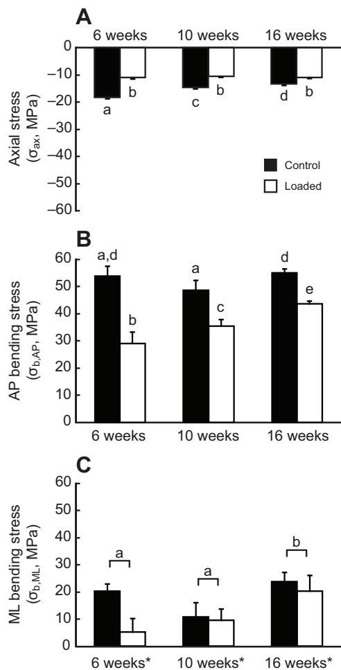
Fig. 7. Stress calculations for the loaded and control tibiae under a 9 N axial compressive load for the 6-, 10- and 16-week-old mice. (A) Axial stress, \sigma_{ax} , (B) anterior-posterior bending stress, \sigma_{b,AP} , and (C) medial-lateral bending stress, \sigma_{b,ML} . Values shown are means \pm 1 s.d. Data for the control and loaded tibiae are shown in black and white, respectively. Different letters above the bars or bracketed pairs of bars indicate significant differences in the means by linear mixed model with repeated measures, followed by pairwise comparisons with Bonferroni correction ( P < 0.05 ). Letters and brackets above the pairs of data bars in C indicate main effect differences with age. Asterisks (*) next to the age group labels in C indicate a main effect difference between the loaded and control limbs across the three age groups corresponding to a general decrease in \sigma_{b,ML} in the loaded tibiae.
