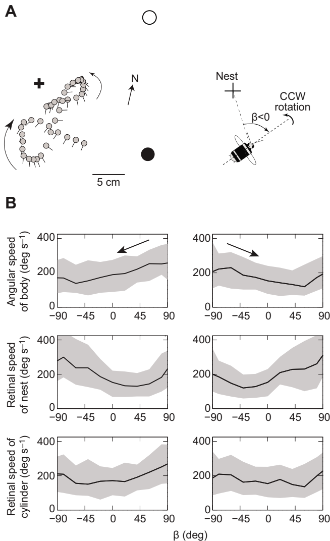
Fig. 5. Pivoting parallax during loops. (A) A pair of CW and CCW loops recorded at 50 frames s -1 . +, nest; the large black and white circles are 20 cm high cylinders. The cartoon on the right demonstrates the convention used for the variables. For CW rotations, \beta (body orientation relative to nest) is positive during turns to the nest. For CCW rotations, \beta is negative. (B) Top row: median angular speed of the body plotted against the angle of the body during 92 CW (left) and 93 CCW (right) loops over the range -90 to +90 deg. The shaded area is the IQR. Bins are 20 deg wide. The arrow denotes the direction of travel through the loop. Centre row: same data showing the median speed of the image of the nest across the retina and the IQR estimated from the orientation of the body. Bottom row: median speed and IQR of the more northerly cylinder (white circle) across the retina. Shaded areas indicate the IQR of the data. (C) Median angular speeds of the retinal image of different positions around the nest and landmarks for CW (upper two panels) and CCW (lower two panels) turns towards (first and third panels) and away from (second and fourth panels) the nest. Data are shown in greyscale from white (low, 120 deg s -1 ) to black (high, 320 deg s -1 ) from the same loops as in B. +, nest; the white and black circles indicate 20 cm high cylinders. Further details are given in Materials and methods.
