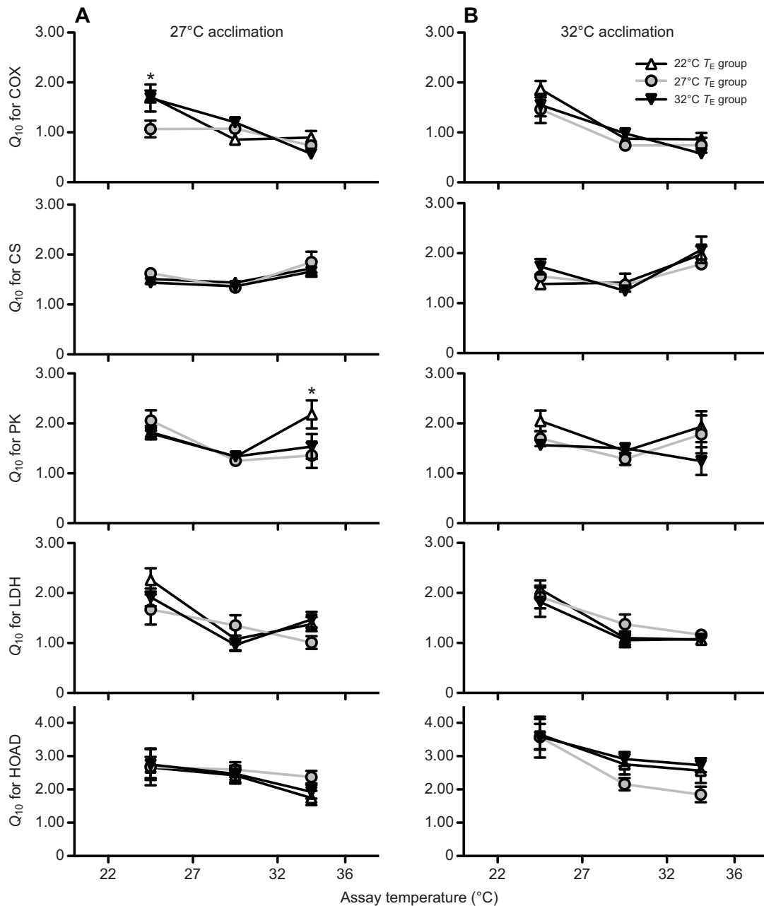
Fig. 9. The effects of embryonic temperature ( T_E ) on the temperature sensitivity of metabolic enzymes in the muscle. Temperature coefficients ( Q_{10} ; the fold-change in activity for a 10°C increase) were calculated between assay temperatures ( T_a ; see Materials and methods). T_E affected Q_{10} in zebrafish acclimated to 27°C (but not in those acclimated to 32°C) for cytochrome c oxidase (COX) and pyruvate kinase (PK), but there was no effect of T_E on Q_{10} for citrate synthase (CS), hydroxyacyl-coA dehydrogenase (HOAD) or lactate dehydrogenase (LDH). Acclimation to a warmer temperature increased Q_{10} for HOAD between assay temperatures of 22 and 27°C, reflecting an increased sensitivity to cooler temperatures ( n=10 per treatment group).
