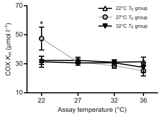
Fig. 4. Embryonic temperature ( T_E ) affected the kinetics of cytochrome c oxidase (COX) in the muscle for its substrate, reduced cytochrome c. Kinetics are represented by substrate affinity ( K_m ), the concentration of reduced cytochrome c that supports 50% of maximal activity. There was a significant interaction between T_E and assay temperature ( T_a ) on K_m in fish acclimated to 27°C ( F_{6,108}=2.36 , P=0.035 ), which are shown in the figure. There was also a significant main effect of T_E on K_m in fish acclimated to 32°C ( F_{2,108}=4.91 , P=0.009 ; data shown in Table 4). The asterisk represents a significant difference between the 27°C T_E group and both other T_E groups in Bonferroni pairwise comparisons ( n=10 per treatment group).
