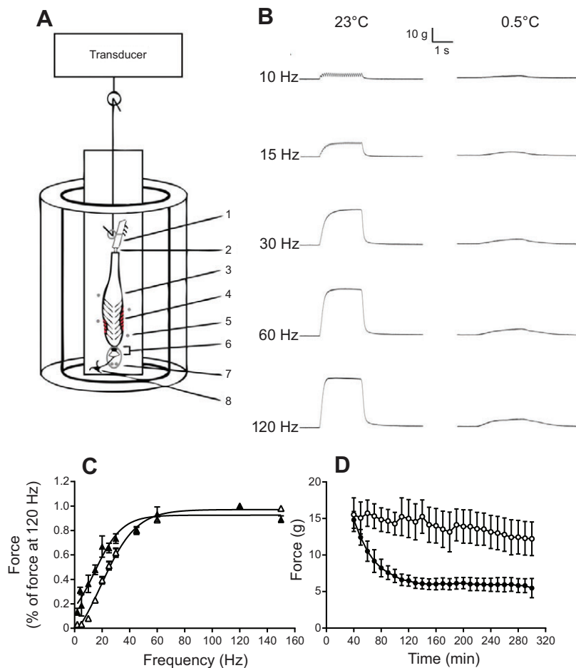
Fig. 2. Schematic diagram of the muscle preparation from the hindleg of L. migratoria and control series of tetanic force production. (A) The muscle preparation consists of the tibia (1), femur (3), coxa and trochanter (6) and nerve ending from the methathoracic ganglion (8). The coxal end is fastened with suture to two metal pins (7) embedded perpendicularly in a vertically oriented Plexiglas plate that also contained the wire electrodes (5) for field stimulation. The tibial end was fastened to a stainless steel hook connected to a force transducer. To expose the muscle tissue to the electrical field stimulation, two small incisions were made in the exoskeleton (4). To avoid the build-up of force in the bending springs positioned in the joint section and to secure a straight pull in the transducer, the cuticle in this area was removed and the tendons were exposed (2). The whole preparation was submerged in a water-jacketed glass chamber containing standard locust saline.
