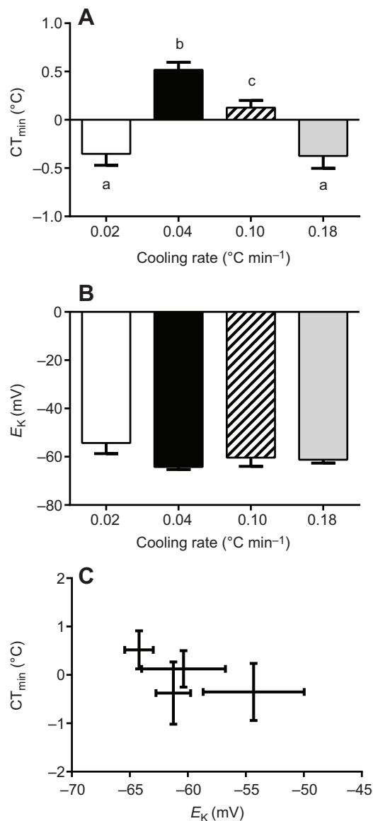
Fig. 1. CT_{min} and E_K measurements of Locusta migratoria at four different cooling rates (0.02, 0.04, 0.1 and 0.18°C min -1 ). (A) Chill coma temperature ( CT_{min} ) was assessed as the temperature at which the animal was paralysed by cold and was non-responsive. Bars represent means \pm s.e.m. of 25 locusts for each cooling rate treatment. Different letters indicate groups that differ significantly. (B) Equilibrium potential of K + ( E_K ) at -1°C for four different cooling rates (0.02, 0.04, 0.1 and 0.18°C min -1 ). (C) CT_{min} plotted against E_K values at -1°C. Values are means \pm s.e.m. Additional information can be found in supplementary material Figs S1–S3.
