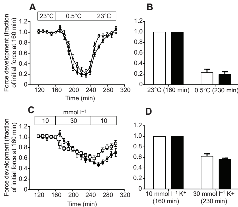
Fig. 3. Tetanic force production at different temperatures and [\text{K}^+] with and without TTX. (A) Tetanic force production was elicited every 10 min in preparations with (filled circles) and without TTX (open circles). Force production was normalized to that obtained at 160 min and temperature was lowered gradually from 23^\circ\text{C} to 0.5^\circ\text{C} from 160 min. The experimental temperature ( 0.5^\circ\text{C} ) was reached within 50 min and the preparation was allowed to stabilize for the following 30 min before being returned quickly to 23^\circ\text{C} at 240 min. Symbols represent means \pm s.e.m. of five to six preparations in each treatment. (B) Tetanic force production at 0.5^\circ\text{C} normalized to force at 23^\circ\text{C} for TTX-treated (filled bars) and non-treated (open bars) preparations. Bars represent means \pm s.e.m. of five to six preparations in each treatment. (C) Tetanic force production was elicited every 10 min in preparations with (filled squares) and without TTX (open squares). Force production was normalized to that obtained at 160 min and [\text{K}^+]_o was increased from 10 to 30 \text{ mmol l}^{-1} from the 160th minute. The experimental \text{K}^+ concentration ( 30 \text{ mmol l}^{-1} ) was maintained at this level for 80 min before returning to 10 \text{ mmol l}^{-1} at the 240th minute. Symbols represent means \pm s.e.m. of six preparations in each treatment. (D) Tetanic force production at 30 \text{ mmol l}^{-1} \text{ K}^+ normalized to force at 10 \text{ mmol l}^{-1} \text{ K}^+ for TTX-treated (filled bars) and non-treated (open bars) preparations. Bars represent means \pm s.e.m. of six preparations in each treatment.
