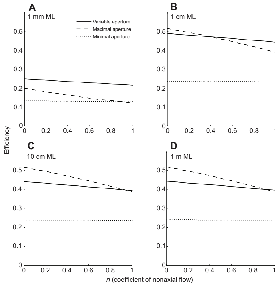
Fig. 7. Effects on whole-cycle hydrodynamic efficiency of n , the coefficient of nonaxial flow. Theoretical results for squid of (A) 1 mm ML, (B) 1 cm ML, (C) 10 cm ML and (D) 1 m ML. Models with a constant small aperture area (dotted line), a constant large aperture area (dashed line) and a dynamically varying aperture area (solid line) are shown. This coefficient can also represent pressure effects if permitted to range below 0 and above 1; model runs with values of -0.1 and 1.1 (not shown) were not remarkably different.
