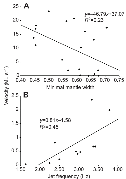
Fig. 2. Kinematics of paralarval D. gigas swimming, from standard 30 frames s^{-1} video clips. (A,B) Velocity plotted against the minimal mantle width (A; ratio of fully contracted to fully expanded mantle, smaller numbers indicate more contraction) and frequency of contraction (B); single fast jets were excluded, because frequency cannot be calculated.
