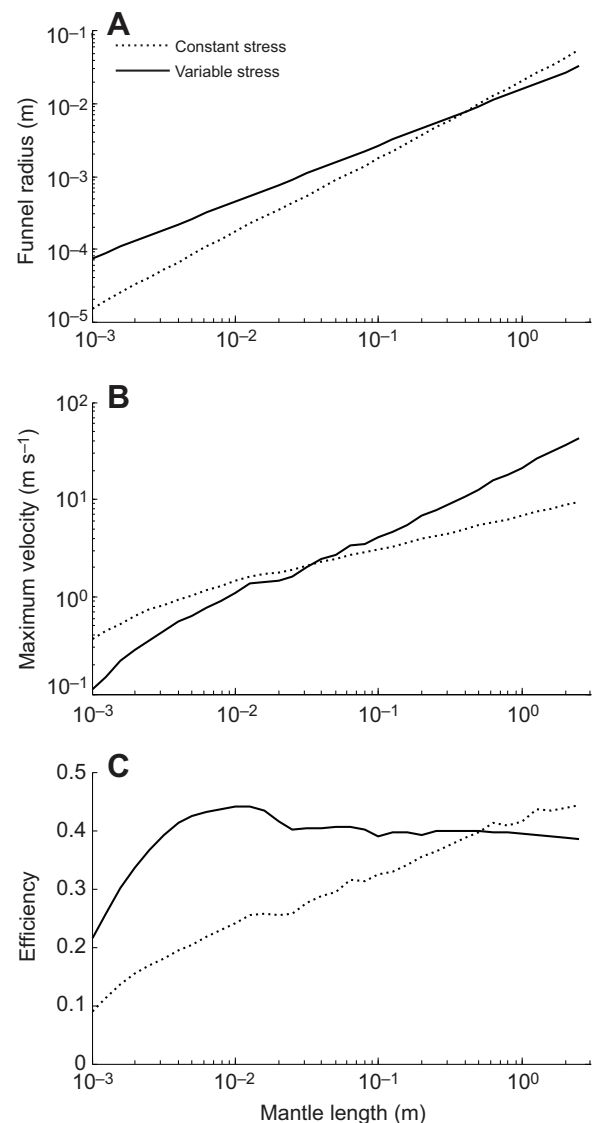
Fig. 5. Size-dependent variation in jetting when variables are set by regressions with a dynamically varying aperture, allowing stress to vary (solid lines), compared with when funnel radius is controlled to maintain a constant stress of 2.5 \times 10^5 N m ^{-2} (dotted lines). (A) Size-dependent variation in funnel radius. (B,C) Theoretical results of using this radius for maximal squid velocity at the peak of a single jet (B) and hydrodynamic efficiency (C).
