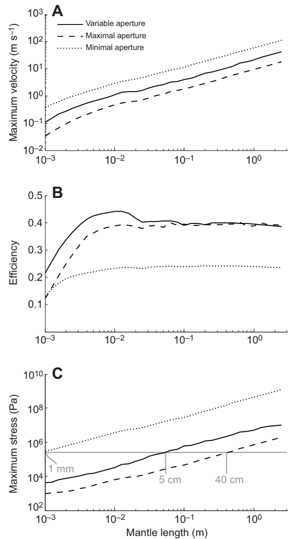
Fig. 4. Size-dependent scaling of squid jet propulsion and the effect of jet aperture area. Theoretical results for (A) maximal squid velocity at the peak of a single jet, (B) hydrodynamic efficiency summed over 10 jet cycles, and (C) maximal stress on the mantle muscle at the peak of a single jet. Models with a constant small aperture area (dotted line), a constant large aperture area (dashed line) and a dynamically varying aperture area (solid line) are shown. A horizontal gray line in C indicates a maximal muscle stress of 2.5 \times 10^5 \text{ N m}^{-2} . Mantle lengths at which this stress is reached for each of the three models are given in gray.
