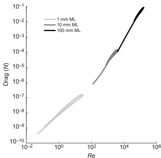
Fig. 9. Drag as a function of Reynolds number for three sizes of squid. Data for 10 cycles of contraction and refilling are plotted for each squid (1, 10 and 100 mm ML); loops emerge because drag depends on both Re and squid velocity.
