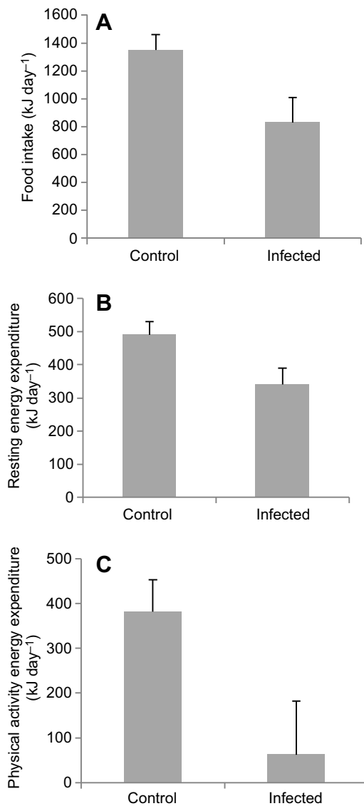
Fig. 2. Impact of 16 days infection with a nematode parasite on the energy budget of grouse. (A) Food intake ( \text{kJ day}^{-1} ), (B) resting energy expenditure ( \text{kJ day}^{-1} ) and (C) physical activity energy expenditure ( \text{kJ day}^{-1} ). Infected grouse show large reductions in all three parameters relative to uninfected controls. Figure drawn from data presented in Delahay et al. (1995). The values are means \pm s.d.
