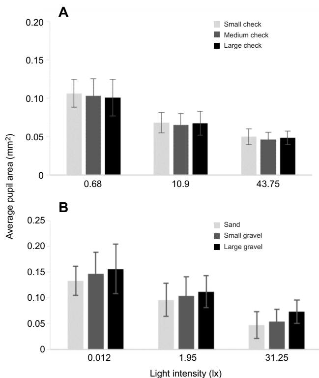
Fig. 3. Average pupil areas on experimental substrates. (A) Experiment 1: pupil dilation for skates placed on artificial checkerboards. The skate pupil constricted with increasing light intensity but did not respond to changes in spatial frequency of the checkerboards (there was no significant difference between check sizes; there was a significant difference between light intensities; see Results for details). (B) Experiment 2: pupil dilation for skates allowed to bury in natural substrates, with only their eyes protruding. In addition to reacting to light intensity, the skate pupil constricted/dilated in response to the spatial frequency of the substrate: the smaller the substrate spatial frequency, the more constricted the pupil. This effect was statistically significant (see Results for details). Note that different dilation:constriction ratios in A and B are due to skate size differences.
