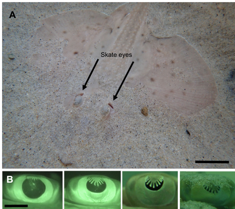
Fig. 1. Eyes of the skate Leucoraja erinacea . (A) A skate partially buried in sand. Scale bar: 8 cm. (B) Close-ups of skate eyes showing the range of dilation/constriction states from fully dilated (left) to near-constricted (right), revealing an elaborate, finger-like shape. Scale bar: 1 cm.
