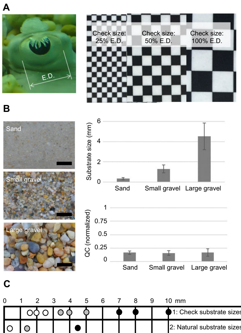
Fig. 2. Substrates used in experiments 1 and 2.
