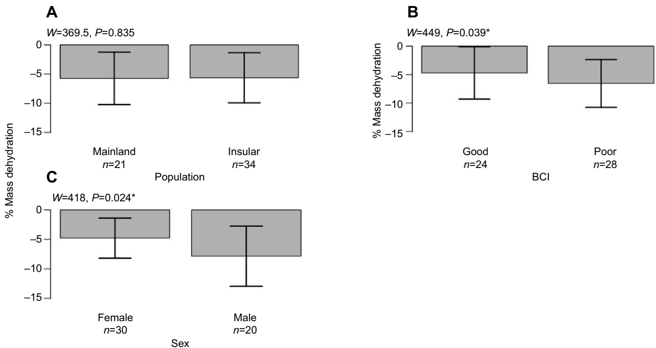
Fig. 4. Bar graph plots of drinking threshold. Drinking threshold is the dehydration threshold for drinking and was defined as the percentage body mass lost to dehydration at which an animal first drinks fresh water. (A) Drinking threshold of mainland ( n=21 ) and insular ( n=34 ) populations of cottonmouth snakes. (B) Drinking threshold of cottonmouth snakes in good ( n=24 ) and poor ( n=28 ) condition. (C) Drinking threshold of female ( n=30 ) and male ( n=20 ) cottonmouth snakes. Data were compared with Wilcoxon rank sum tests. Bar graph plots represent the mean \pm s.d. *Statistical significance at the 0.05 alpha level.
