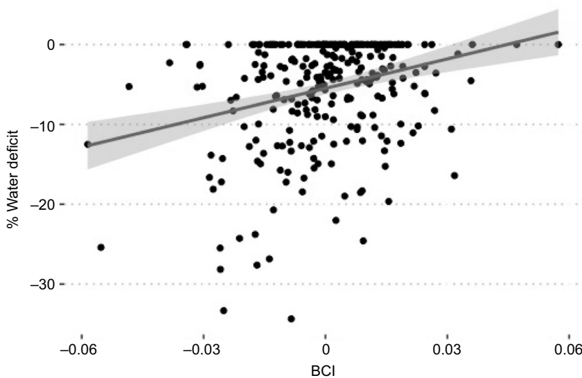
Fig. 3. Scatterplot of body condition index (BCI) and apparent water deficit. Results of the field study of the hydration status of insular cottonmouth snakes ( n=290 ) showing the linear regression of BCI and apparent water deficit of individuals (measured as the percentage change in mass from drinking) ( F_{1,288}=24.34 , P<0.001 ). Solid line indicates line of regression ( y=1.23x-0.05 , R^2=0.08 ) and gray shading represents the 95% confidence interval.
