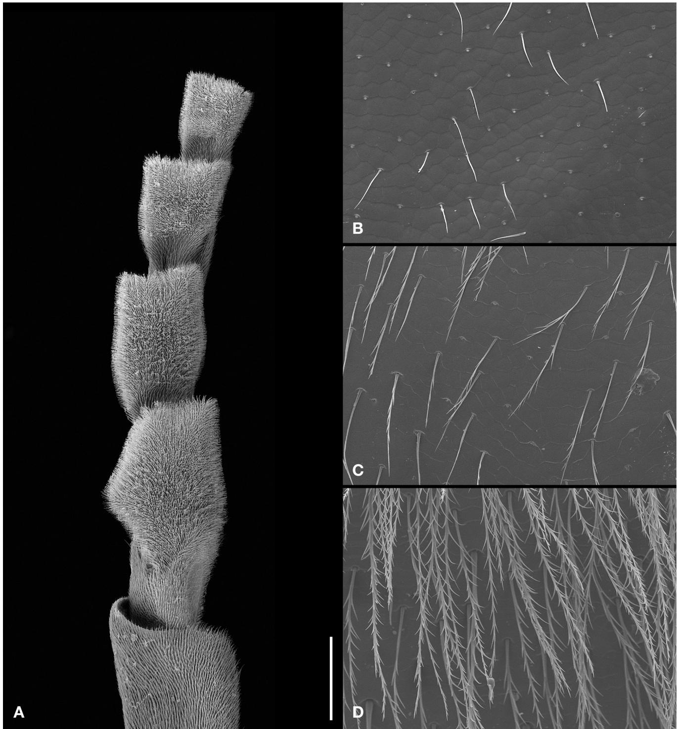
Figure S3. Tarsus of Stylops ovinae (A) and hairiness of the abdominal tergites II–IV of a stylized Andrena vaga (B–D), SEM-micrographs. (A) Prothoracic leg, ventral view (modified from Pohl & Beutel, 2004). (B) Abdominal tergite II. (C) Abdominal tergite III. (D) Abdominal tergite IV. Scale bar: 100 \mu m.
