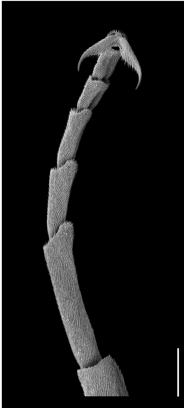
Figure S4. Mogenilla moldrzyki (Mogenillidae), male, tarsus of metathoracic leg, ventral view, SEM-micrograph (modified from Pohl & Beutel, 2004). Scale bar: 100 \mu\text{m} .
