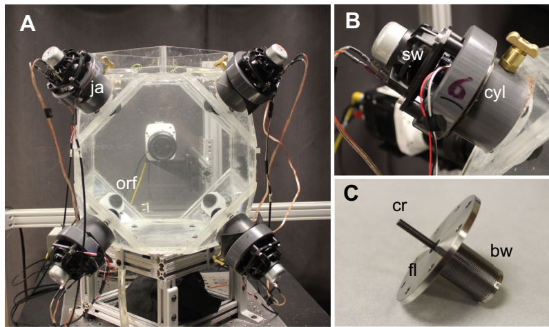
Fig. 1. Images of the turbulence tank, a jet actuator and the bellows assembly that displaces fluid in the jet actuator cylinders. (A) In the whole-tank view, four of the eight jet actuators (ja) and some of the black domed orifices (orf) of the tank are visible. (B) The close-up of the jet actuator shows the subwoofer speaker (sw) and wires leading to the accelerometer on the rod connecting the speaker to the bellows inside the cylinder (cyl). (C) The bellows (bws) assembly shows the connecting rod (cr) and the flange (fl), which is the lid of the fluid cylinder. The flange and cylinder are sealed with a rubber gasket (not shown) and the cylinder is connected to the tank wall with glue and fasteners.
